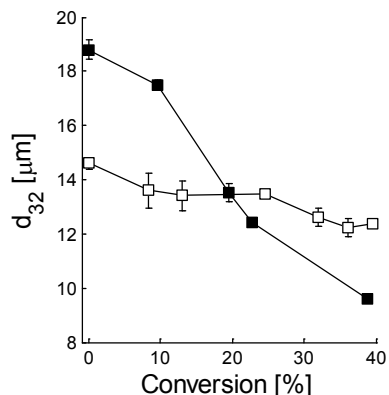
Figure 3.5. The area mean particle diameter ( d_{32} ) plotted as a function of glucan conversion during bioreactor enzymatic hydrolysis at an agitation rate of 300 rpm, as reported in Paper I . White and black squares represent steam pretreated spruce and giant reed, respectively.
