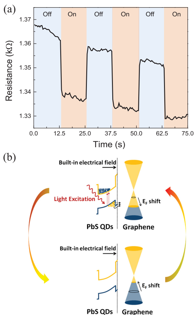
FIG. 2. (a) Temporal resistance response of a typical hybrid PbS quantum dots/graphene device while switching the laser light on and off, taken at gate voltage of V_g = -10 V and source-drain bias of V_{sd} = 100 \mu\text{V} . (b) Schematic diagram of the photoresponse mechanisms of hybrid device under laser illumination and in the dark.
