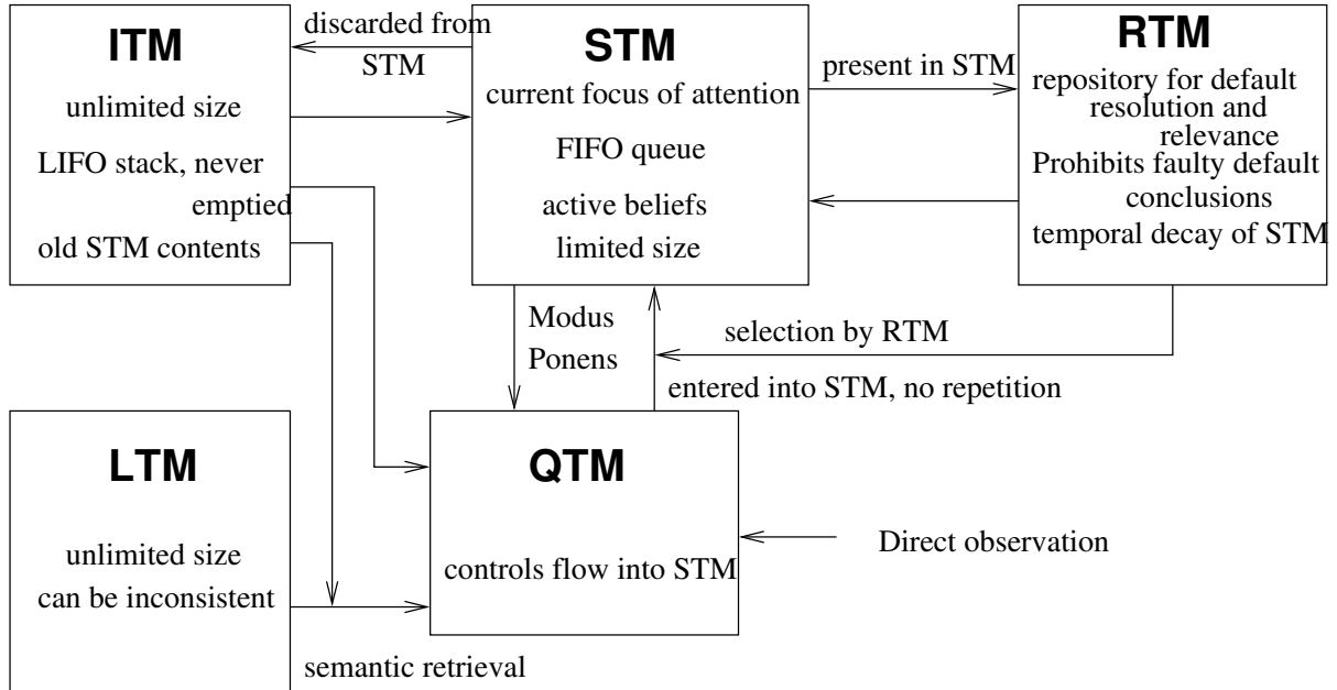
Figure 1: The memory model from [8].
