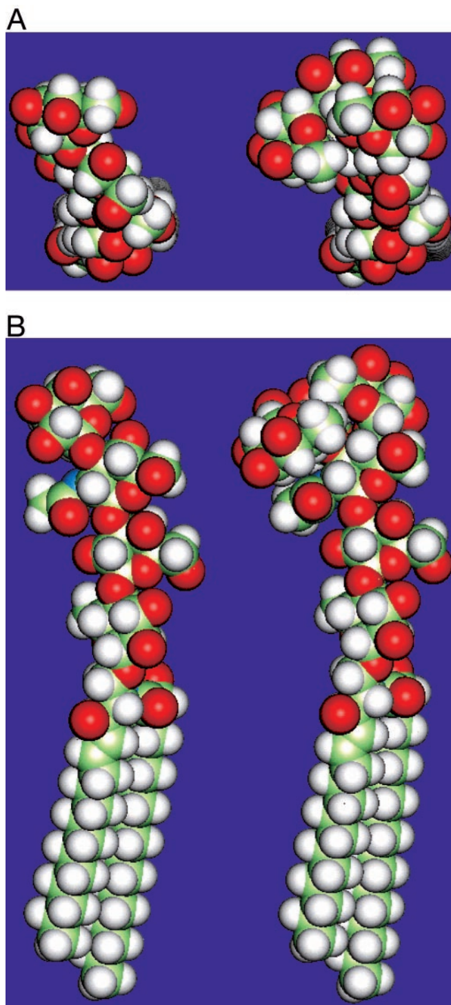
FIG. 11. Minimum energy conformers of the H. pylori binding lactotetraosylceramide (Gal \beta 3GlcNAc \beta 3Gal \beta 4Glc \beta 1Cer, left) and the Le b -6 glycosphingolipid (Fuc \alpha 2Gal \beta 3(Fuc \alpha 4)GlcNAc \beta 3-Gal \beta 4Glc \beta 1Cer, right) (B). The top charts (A) show the same structures viewed from above. The Glc \beta 1Cer linkage is shown in an extended conformation. A detailed comparison between these two structures is made in the text.
