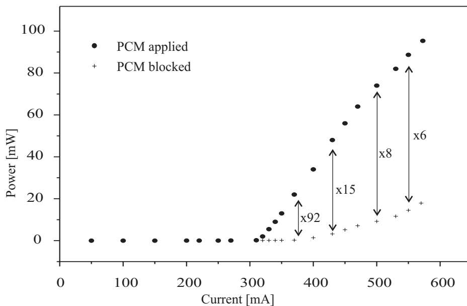
Figure 4. Power-current characteristics from the 50\ \mu\text{m} core diameter fiber when the feedback system is applied (dots) vs. when the laser runs freely (cross hairs). The feedback system ensures a large conversion of multi-mode radiation into a high-quality almost diffraction limited beam that couples well to the fiber.
