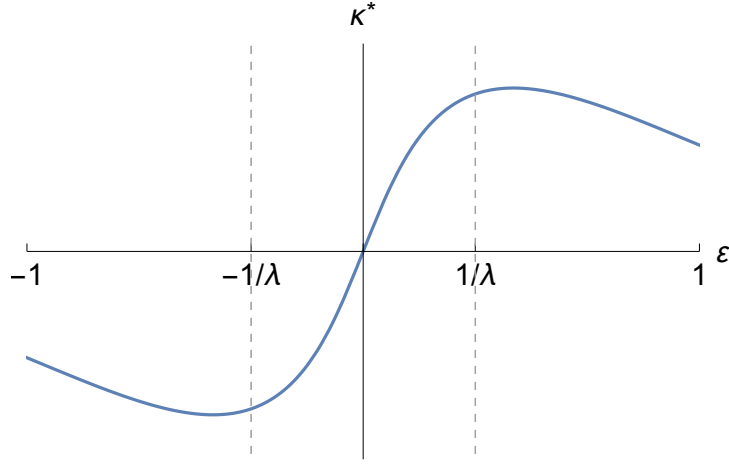
Figure 3: Optimal taste for three-state environments. Each environment has three equiprobable states that yield objective payoff differences x \in \{-1, \varepsilon, 1\} . The DM has a logistic SCR with imprecision parameter \lambda . For environments with \varepsilon \in [-1/\lambda, 1/\lambda] , the optimal taste is increasing in \varepsilon , even though the SCR is not moderate over the whole X \times K .
