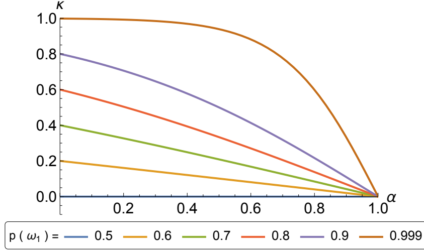
Figure 8: Optimal taste for different levels of base-rate neglect \alpha in binary environments. The two states of the world \{\omega_1, \omega_2\} have objective-payoff differences x(\omega_1) = 1 and x(\omega_2) = -1 . Plots for environments with different p(\omega_1) .
