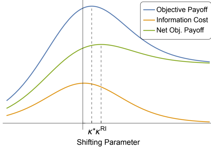
Figure 6: Optimisation over shifting parameters for the adapted-preference model and the rational-inattention model. The adapted-preference agent receives the full “Objective Pay-off”, while the rationally inattentive agent has to pay some information cost for the same amount of bias, receiving “Net Objective Payoff.” When they are both optimising, the rationally inattentive agent biases her SCR more than the adapted-preference agent to save on information costs.
