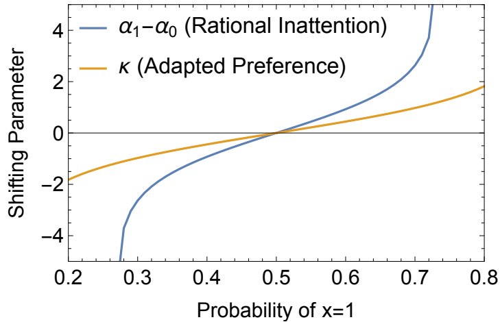
Figure 7: Optimal shifting parameters in binary environments for the adapted-preference model and the rational-inattention model. The two states of the world \{\omega_1, \omega_2\} have objective-payoff differences x(\omega_1) = 1 and x(\omega_2) = -1 . Plots for environments with different p(\omega_1) .
