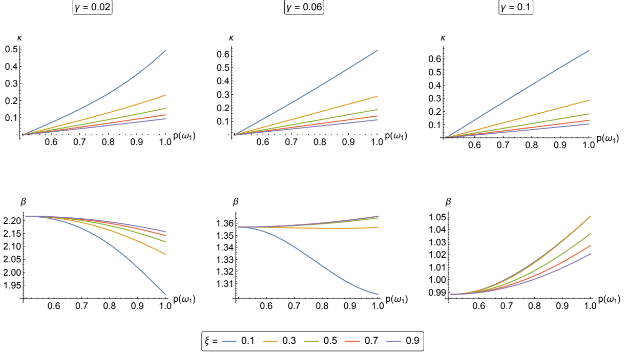
Figure 4: Optimal taste \kappa and logit precision \beta in various binary environments when the DM can adjust taste and logit precision at cost \gamma\beta^2 + \xi|\kappa|^2 . The two states of the world \omega_1, \omega_2 have objective payoff differences x(\omega_1) = 1 and x(\omega_2) = -1 . Environments vary in their probability p(\omega_1) .
