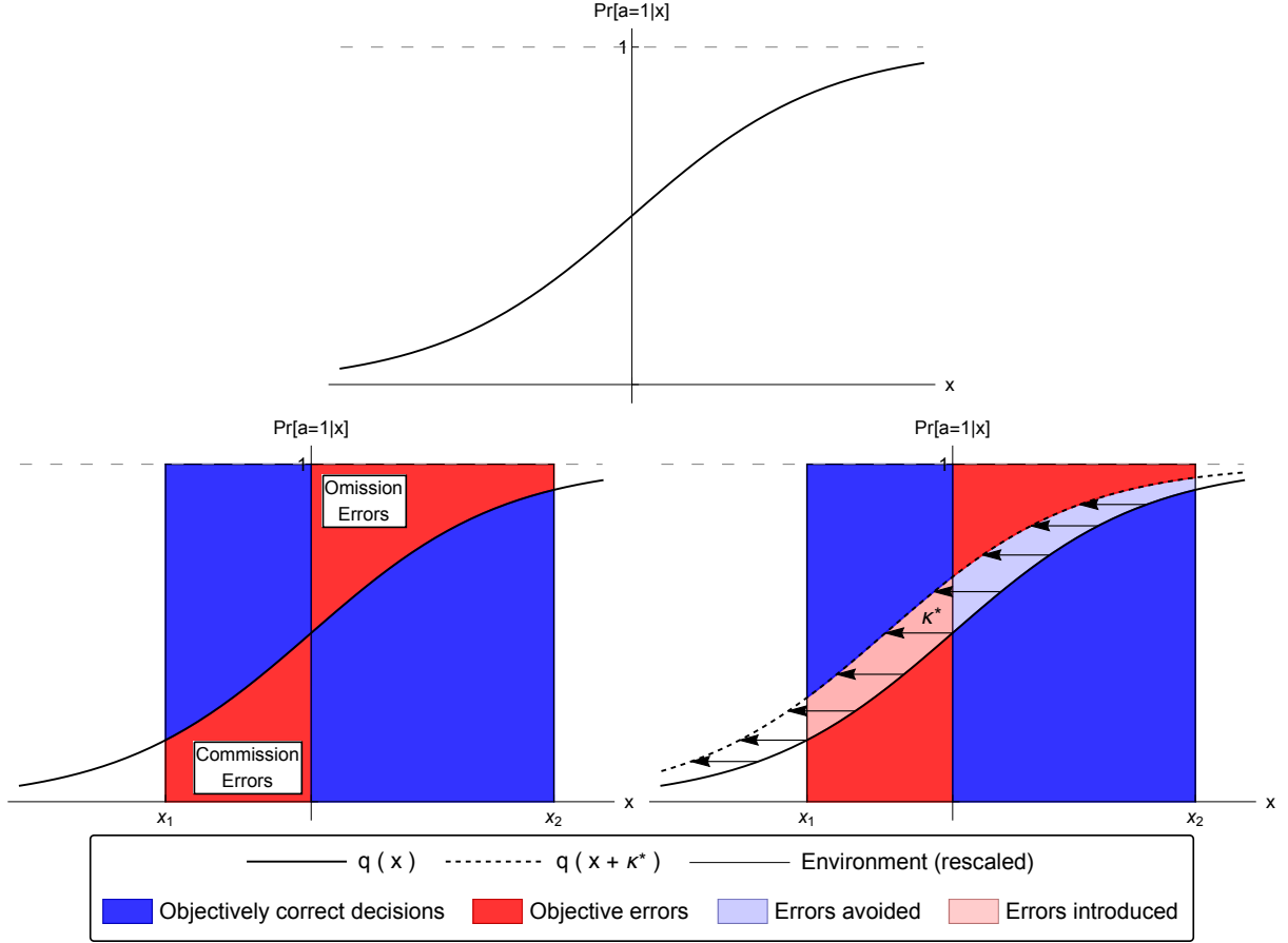
Figure 2: How tastes correct mistakes. Top panel: the DM's stochastic choice rule with a neutral taste ( \kappa = 0 ). Bottom left panel: The DM is using her SCR to act in an environment where the objective-payoff difference x is uniformly distributed between x_1 and x_2 . In this environment, the DM is making both commission and omission errors. Bottom right panel: With the optimal taste \kappa^* > 0 , the DM makes some additional commission errors, but also avoids some omission errors. The value of the omission errors avoided is higher than the value of the commission errors introduced and the DM is better off with taste \kappa^* .
