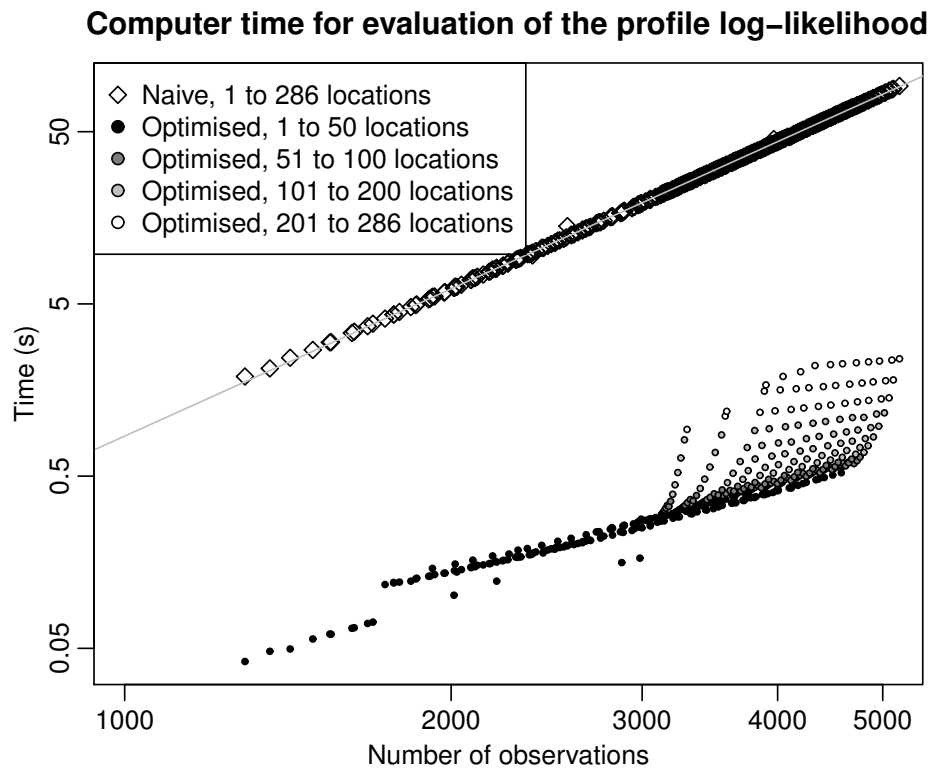
FIGURE 5. Comparison of the time needed for one evaluation of the naïve profile likelihood (9) and simplified version (12). The full dataset, 5182 observations from 286 locations and 280 time points, was divided into smaller pieces by dropping either locations and/or time-points to examine how fast the evaluation time would grow as the dataset was expanded. Evaluation time for the full likelihood grows as N^{2.8} (the fitted line) close to the expected theoretical value of O(N^3) . For a fixed number of locations evaluation time for the simplified version grows considerably slower than N^3 .
