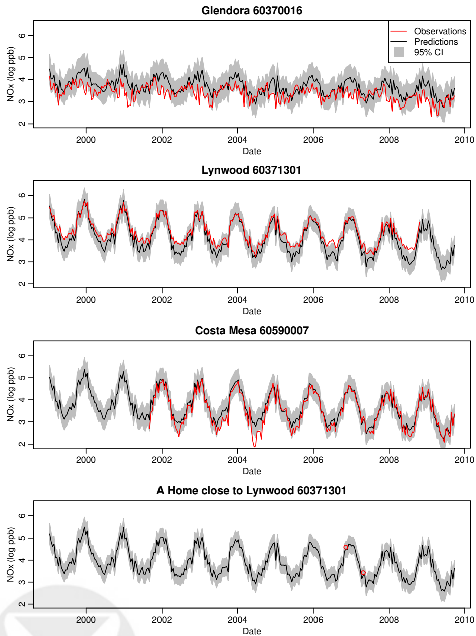
FIGURE 6. Example of cross-validated predictions of the log-transformed 2-week average \text{NO}_x concentrations at three AQS monitors and one home site in the Los Angeles area. Observations, predictions, and 95% prediction intervals are shown.
