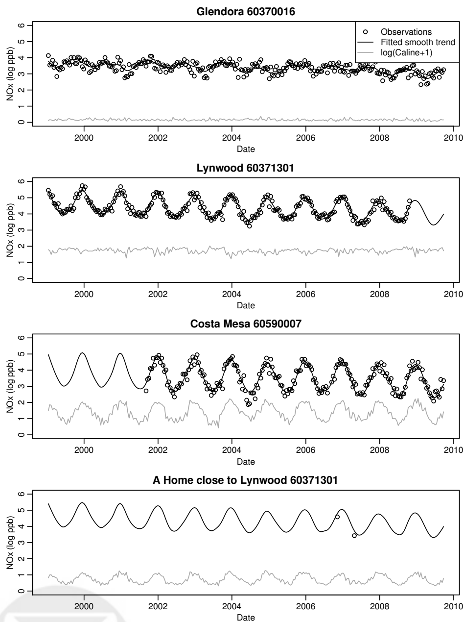
FIGURE 1. Example time series of log-transformed 2-week average \text{NO}_x concentrations at three AQS monitors and one home site in the Los Angeles area. The fit of our smooth temporal basis functions to the data, and the transformed 3km buffer Caline predictions are also shown. For the home site we have used the smooth temporal fit at the closest AQS monitor.
