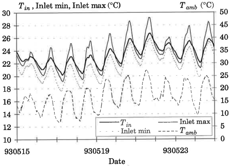
Figure 7.18 The hourly average inlet air temperature, The ambient temperature and the inside temperature at the four inlets for the period 930515-930525.
