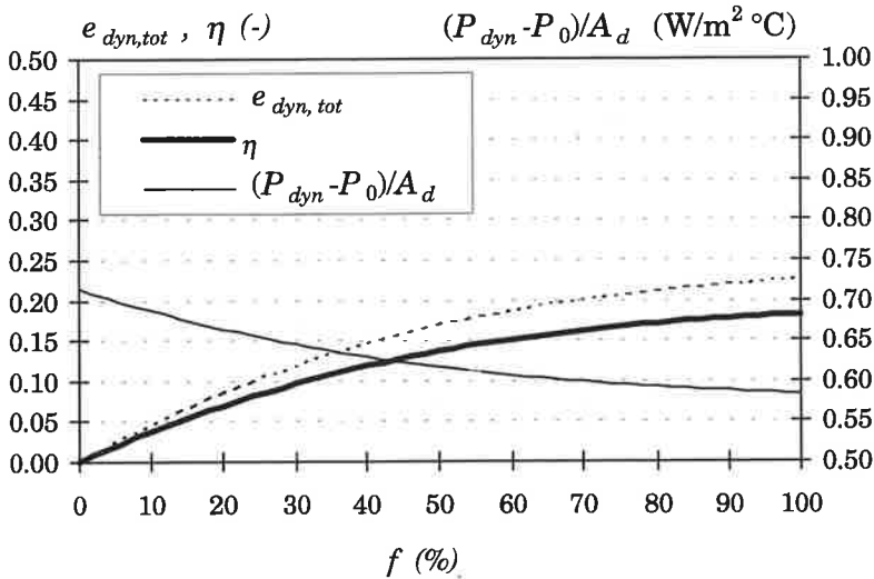
Figure 3.5. The total energy efficiency e_{dyn,tot} , the relative energy saving \eta and the energy loss through conduction and ventilation per square meter (P_{dyn}-P_0)/A_d in the ceiling in the OPTIMA house as a function of the fraction f of the inlet air that passes through the insulation. The calculations are based on H=0.3m , a total air flow Q=53\text{ l/s} and an dynamic area A_d=116\text{ m}^2 .
