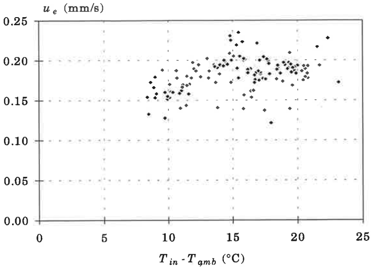
Figure 7.11 The 24h average u_e versus (T_{in} - T_{amb}) for the period 930224-930420 and 930828-931106.
