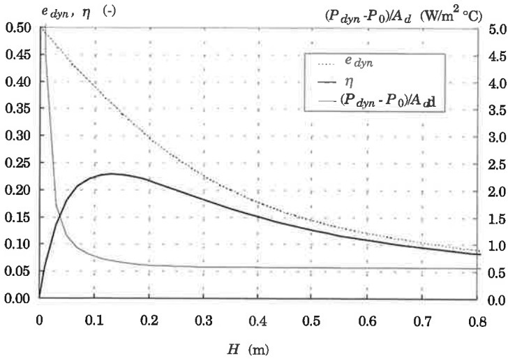
Figure 3.4. The energy efficiency e_{dyn} the relative energy saving \eta and the energy loss through conduction and ventilation per square meter (P_{dyn}-P_0)/A_d in the ceiling in the OPTIMA house as a function of the height of the insulation H . The calculations are based on f=100\% and the total flow 53 \text{ l/s} .
