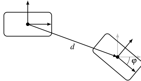
Figure 2: Illustration of the two-dimensional rigid body motion under consideration. The motion of the platform is described by a displacement d and a rotation an angle \phi around the plane normal.
