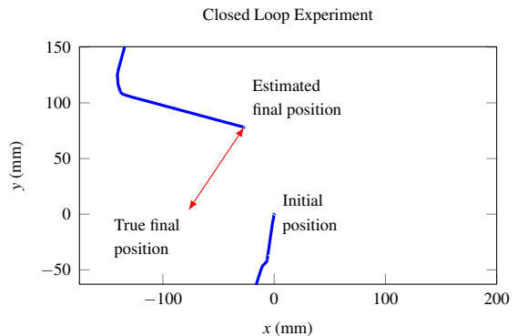
Figure 9: Close-up of the trajectory in Figure 8, showing the initial and final position.
