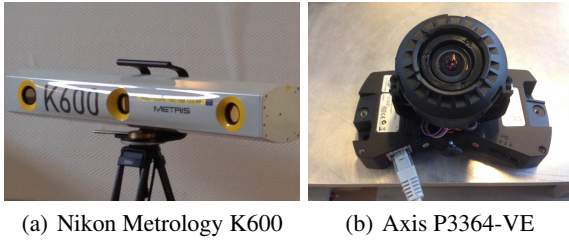
Figure 5: The stationary Nikon Metrology K600 camera (a) used to measure the gold standard positions in the experiments. This is not to be confused with the Axis camera (Axis Communications AB, 2012) (b) that was mounted on the mobile robot and used for the VO.
