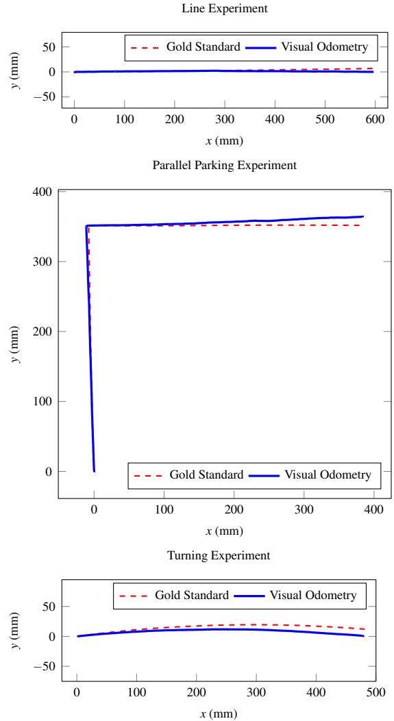
Figure 6: True and estimated positions, using VO. The figure shows the motions in the same order as they are described in the text, i.e. straight line (top), parallel parking (middle), and light turn (bottom). See also Figure 7, where the position errors in relation to travelled distance are shown.
