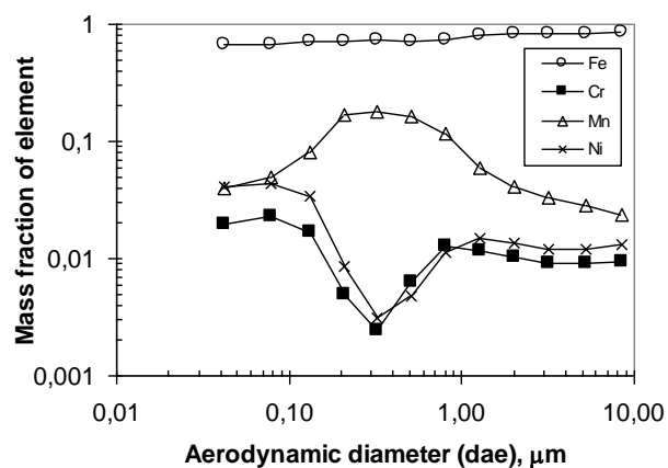
Figure 5. Size-fractionated elemental composition of particles sampled during a background measurement in workshop 3.
