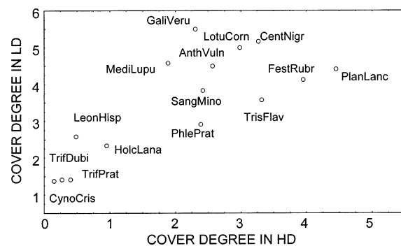
Fig. 6. Relationship between performance of the species in LD plots and HD plots. UK is used as an example.
