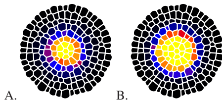
Fig. 9. WUSCHEL equilibrium concentrations in a simulation where the repressive signal is reduced by a factor two (The parameter V_y is set to half its original value for both models). A) Activator model. B) Repressor model. Color coding as in Figure 3.
