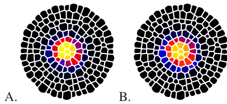
Fig. 8. WUSCHEL equilibrium concentrations in an unperturbed lattice simulation. A) Activator model. B) Repressor model. Color coding as in Figure 3.
