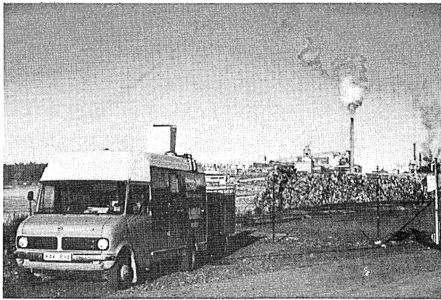
Fig. 1. Mobile DIAL system in a typical measurement situation at a paper mill.
