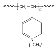
Figure 1: Chemical structure of PVNP.
