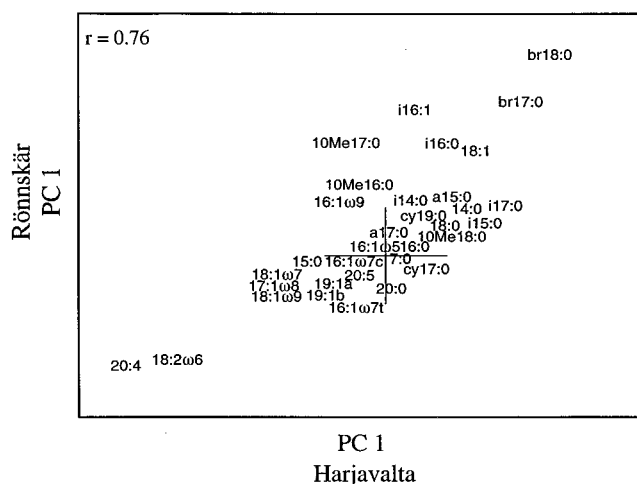
FIG. 5. Loading values for the individual PLFAs of the first principal component (PC 1) from Harjavalta plotted against those from Rönnskär. PLFAs that decreased in proportional abundance at higher pollution levels are found in the lower left corner of the plot, while those that increased are found at the upper right corner.
