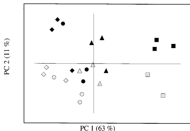
FIG. 2. Score plot of PCA showing the separation of the Harjavalta plots along the first two principal components (PC 1 and PC 2) using PLFA data. Black and grey symbols indicate two different laboratory measurement occasions. Distances from the smelter are indicated as follows: squares, 0.5 km; triangles, 2 km; circles, 4 km; and diamonds, 8 km.
