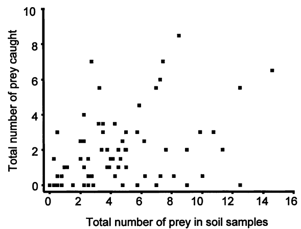
Fig. 6. The total number of prey caught during an experiment (two cages, 20 min) plotted against the total number of invertebrates found in the soil samples from the experiment.
