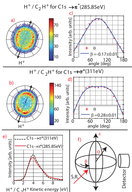
FIG. 1. Experimental data on the \text{H}^+/\text{C}_2\text{H}^+ two-body dissociation channel. The polar plots show the location of the \text{H}^+ ions for (a) the \text{C } 1s \rightarrow \pi^* resonance at 285.85 eV and (b) at 311 eV, which corresponds to the \text{C } 1s \rightarrow \sigma^* resonance. In the lower half of (b) an intensity anomaly can be seen intersecting \vec{\epsilon} , that is due to the injection needle. The direction of the polarization vector is shown in the plots. The \beta -parameter reduces the spherical angle distribution to one numerical value. (c) and (d) show histograms of the zenith angular distribution, \theta , with which \beta has been estimated. The normalized total kinetic energy released to the fragment pair for these two cases is shown in (e). (f) shows that \theta is defined with respect to the polarization vector \vec{\epsilon} . \phi is the azimuth angle. The synchrotron radiation (SR) is perpendicular to \vec{\epsilon} and the detector axis.
