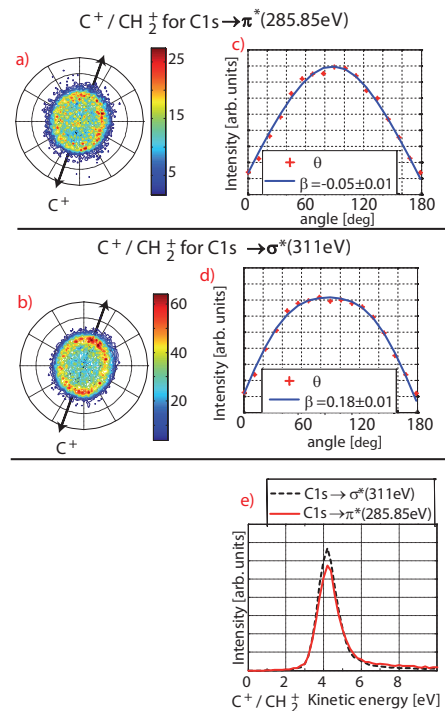
FIG. 2. Experimental data on the \text{C}^+/\text{CH}_2^+ two-body dissociation channel. The polar plots show the location of the \text{C}^+ ions which arrive in coincidence with \text{CH}_2^+ ions for (a) the \text{C } 1s \rightarrow \pi^* resonance at 285.85 eV and (b) at 311 eV. (c) and (d) present the \beta parameters. The total kinetic energy released to the fragments is shown in (e).
