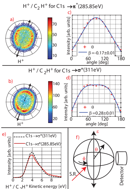
FIG. 1. Experimental data on the \text{H}^+/\text{C}_2\text{H}^+ two-body dissociation channel. The polar plots show the location of the \text{H}^+ ions for (a) the \text{C } 1s \rightarrow \pi^* resonance at 285.85 eV and (b) at 311 eV, which corresponds to the \text{C } 1s \rightarrow \sigma^* resonance. In the lower half of (b) an intensity anomaly can be seen intersecting \vec{\epsilon} , that is due to the injection needle. The direction of the polarization vector is shown in the plots. The \beta -parameter reduces the spherical angle distribution to one numerical value. (c) and (d) show histograms of the zenith angular distribution, \theta , with which \beta has been estimated. The normalized total kinetic energy released to the fragment pair for these two cases is shown in (e). (f) shows that \theta is defined with respect to the polarization vector \vec{\epsilon} . \phi is the azimuth angle. The synchrotron radiation (SR) is perpendicular to \vec{\epsilon} and the detector axis.
