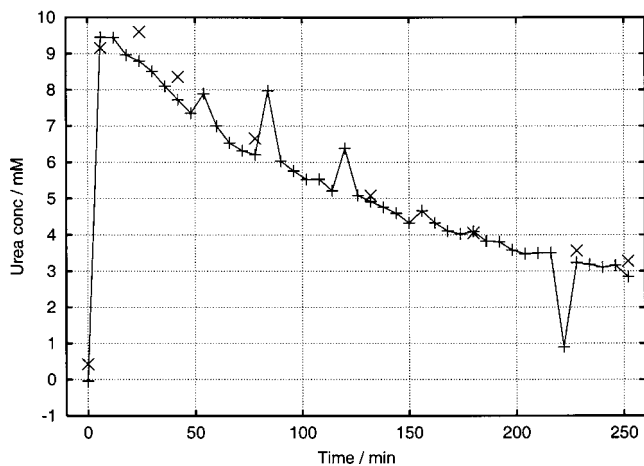
Fig. 3 Representative example of online measurement of urea concentration during treatment. Prediction of urea concentration from NIR spectra based on the three-factor PLS model, “+,” compared with the results of the clinical chemical analysis, “x.”
