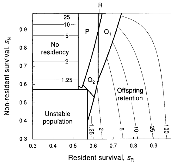
Figure 3: Solutions of the residency game at different values of resident survival s_R and nonresident survival s_N , assuming s_{D1} = s_{S1} = s_{R1} = s_R for both habitat types i = 1 and 2 . Good and poor habitats have productivities r_1 = 0.9 and r_2 = 0.6 , respectively. In the lower left corner, survival is too low to produce a viable population saturating both habitats. Solutions are classified as “no residency” in any habitat (interpretable as complete migration), “offspring retention” where parents and offspring stay resident in both habitats, P denoting partial residency (only parents stay resident in good habitats; interpretable as partial migration), R denoting residency of parents in both habitats, O_1 denoting offspring retention in good habitat only (parents stay and offspring disperse in poor habitats), and O_2 where offspring are retained in good habitat and no residency occurs in poor habitats. In unmarked regions, no pure evolutionarily stable strategy exists. Thick solid lines indicate a change in strategies, and thin contour lines indicate values of the habitat saturation factor H in the areas of “no residency” or “offspring retention.”
