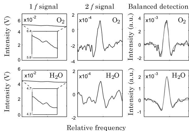
Fig. 2. Typical recorded oxygen and water vapor signals after background subtraction for measurements over an air distance of \sim 20 mm. Insets can be seen in the 1f signal plots enhancing the intensity region of interest for signals due to gas imprint. The balanced-detection 2f signal is shown (black) together with a fitted experimental ideal line shape (gray line). The relative frequency range for both gases corresponds to 35 GHz.
