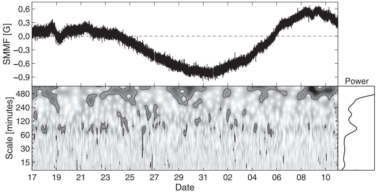
Figure 5. A wavelet analysis of SOHO/MDI SMMF observations. One minute resolution MDI measurements from March 17 to April 10 1999 are shown in the top panel. The data sequence contain 34,852 data points and 1148 (3.2%) data gaps and is given in Gauss. The calculated power spectra in the lower panel cover possible SMMF oscillations with periods from 10 to 500 min. The most distinguishing peaks are found at a period of about 90 min indicated by the power density plot in the lower right panel. The dashed lines indicate the zone of influence. The solid lines show the 95% confidence level.
