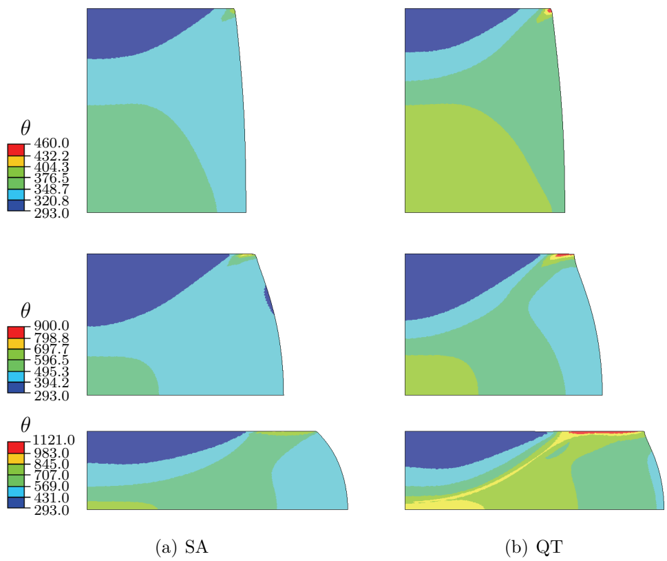
Figure 11: Distribution of absolute temperature \theta at 30, 65 and 100 % deformation as obtained in simulations using the present model.
