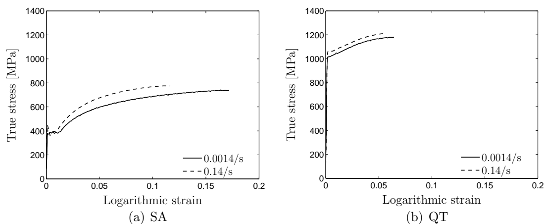
Figure 1: Results of the tensile testing of differently heat treated specimens of 100Cr6 at two different rates of loading.
