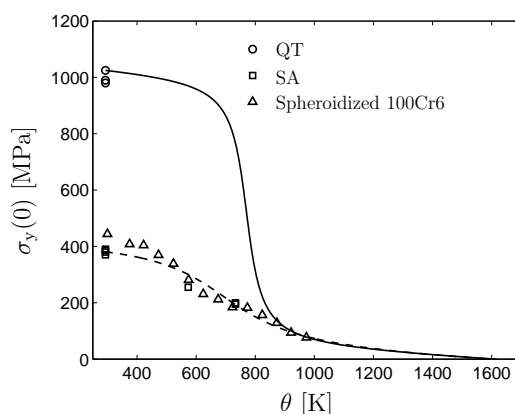
Figure 3: Temperature dependence of the initial yield stress. The experimental results (symbols) are shown together with the fit of the present model for the QT (solid line) and the SA (dashed line) materials, respectively. Results for spheroidized 100Cr6, taken from Löwisch and Dalgic (2006), are shown for comparison.
