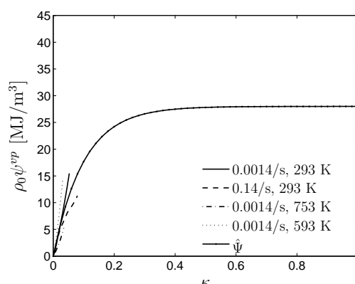
Figure 5: The stored energy of cold work for the SA material obtained in experiments involving different initial temperatures and strain rates. The corresponding results regarding the QT material has the same appearance. \hat{\Psi} denotes the function used in the present model.
