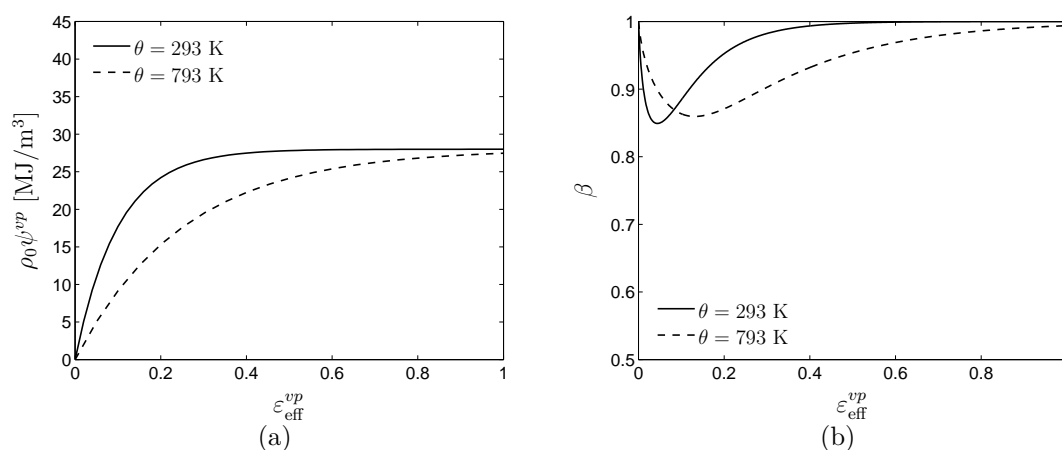
Figure 6: (a) The stored energy of cold work obtained for the SA material at two different constant temperatures. (b) The heat exchange ratio \beta corresponding to the curves in (a).
