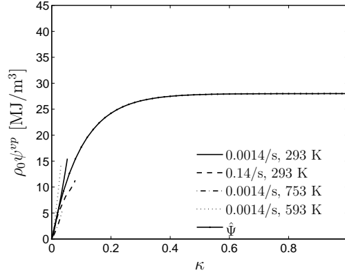
Figure 5: The stored energy of cold work for the SA material obtained in experiments involving different initial temperatures and strain rates. The corresponding results regarding the QT material has the same appearance. \hat{\Psi} denotes the function used in the present model.
