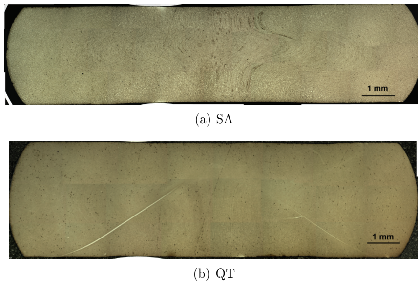
Figure 9: Microscope images of the cross-section of the deformed specimen. (a) The SA material deformed at a rate of approximately 3.5 m/s. (b) The QT material deformed at a rate of approximately 2.5 m/s.
