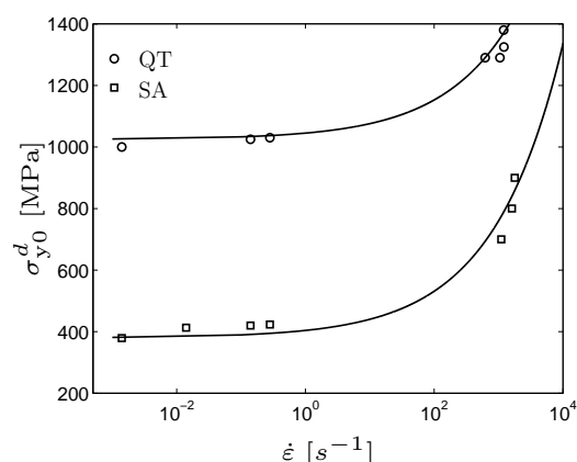
Figure 2: Calibration of the rate dependent initial yield stress of the model (solid lines) against data from experiments (symbols). Note the logarithmic scale on the horizontal axis.
