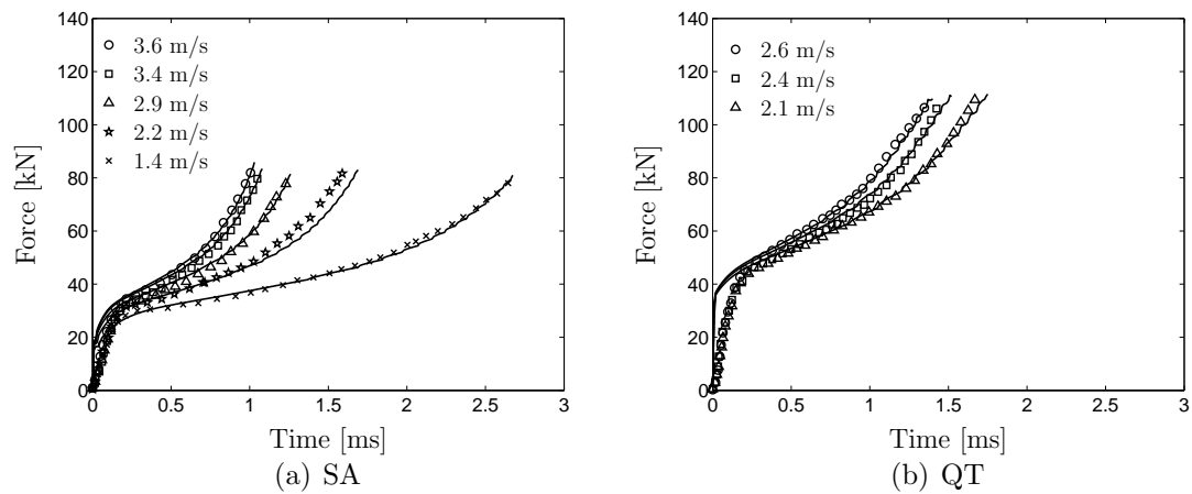
Figure 8: Forming experiments. Simulated response (solid lines) compared with the experimental results (symbols) for different deformation velocities. Note that the velocities of deformation stated here are those used in the simulations as approximations of the mean velocities found in the experiments.
