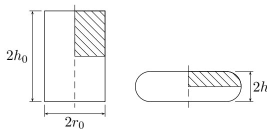
Figure 7: Geometry used in the simulation of the axisymmetric upsetting of a billet. The undeformed geometry is shown at the left and the deformed geometry – with barreling due to friction against the tool – is shown schematically at the right.
