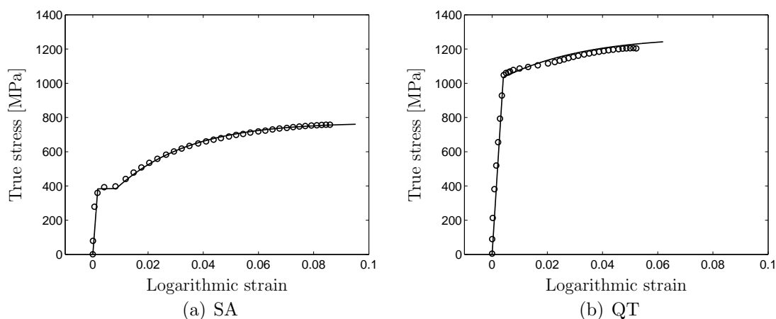
Figure 4: Response according to the model (solid lines) calibrated against experimental results (circles) obtained at a strain rate of 0.14 \text{ s}^{-1} . Note the discontinuous initial hardening of the SA material.
