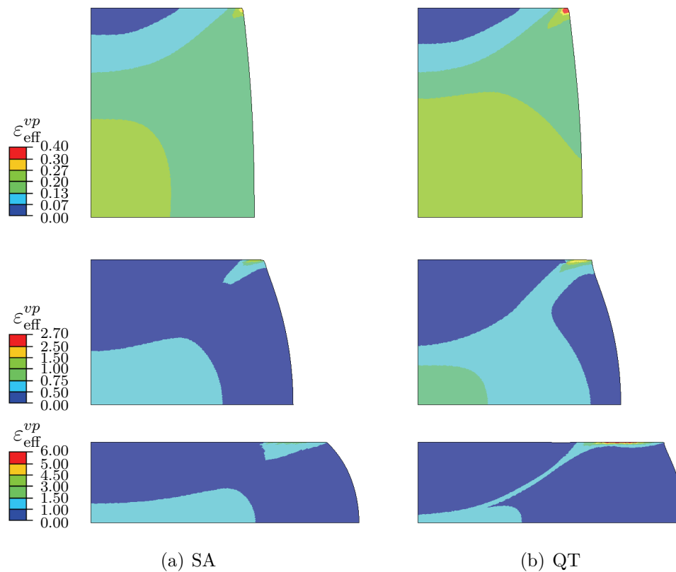
Figure 10: Distribution of effective viscoplastic strain \epsilon_{\text{eff}}^{vp} at 30, 65 and 100 % deformation as obtained in simulations using the present model.
