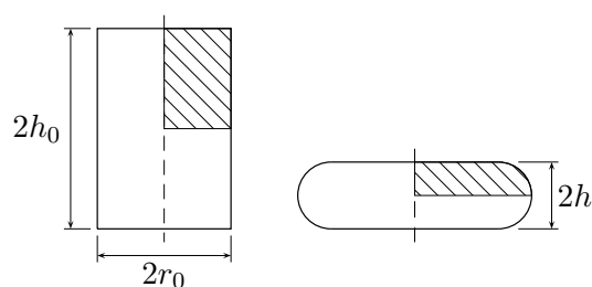
Figure 7: Geometry used in the simulation of the axisymmetric upsetting of a billet. The undeformed geometry is shown at the left and the deformed geometry – with barreling due to friction against the tool – is shown schematically at the right.
