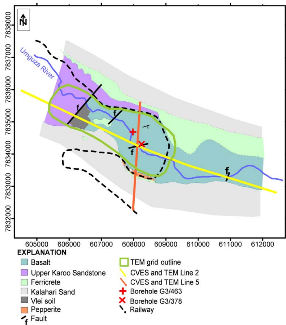
Fig. 3 Field and regional geology map of the Sawmills area, also showing the transient electromagnetic (TEM) grid outline and CVES sounding profiles (lines 2 and 5). The tick marks delineate 1 km
