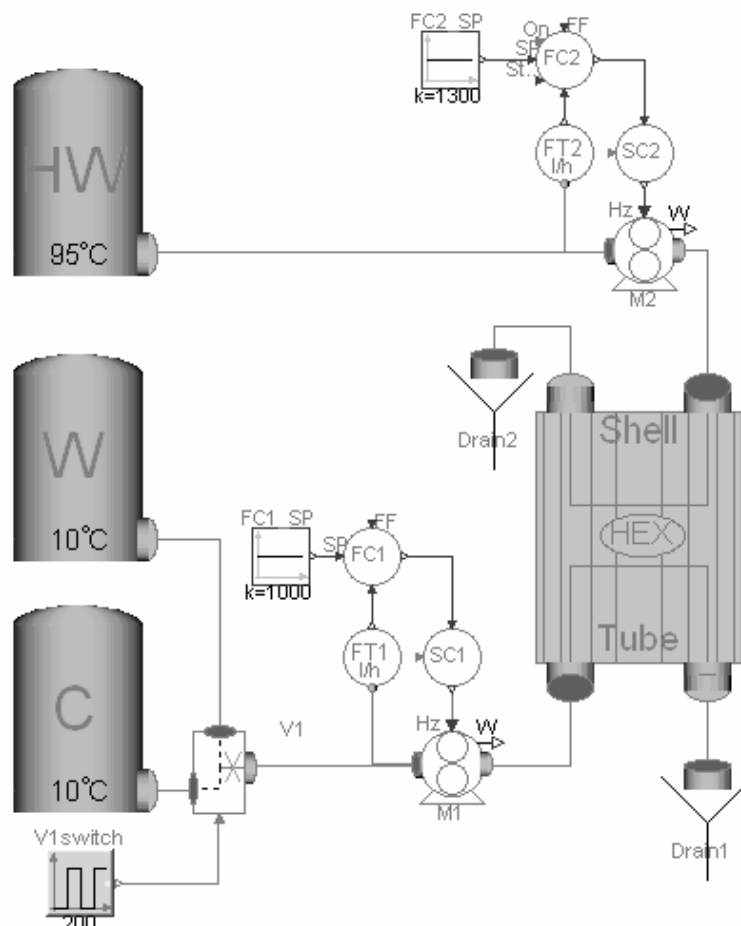
Figure 5. The design of a theoretical experiment as a system of dynamic models, whereof one, denoted “HEX”, is the heat-exchanger model that can be defined as Model I, II or III. Depending on the change-over valve, V1, channel 1 (Tube) is connected to either a water source denoted “W” or a cream source denoted “C”. Channel 2 (Shell) is connected to a hot-water source denoted “HW”. The temperatures in the fluid sources are constant. The flow rate control loop for the tube side (channel 1) includes a sensor (FT1), a PID controller (FC1), a flow set point (FC1_SP), an inverter (SC1) and a pump (M1). The corresponding units on the shell side are FT2, FC2, FC2_SP and M2.
