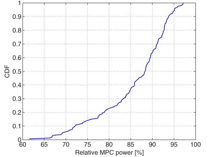
Fig. 2. CDF of the power captured by 40 estimated MPCs, expressed as the percentage of the power calculated from the measured transfer matrix. All 159 measurement positions have been used in calculating the CDF.
