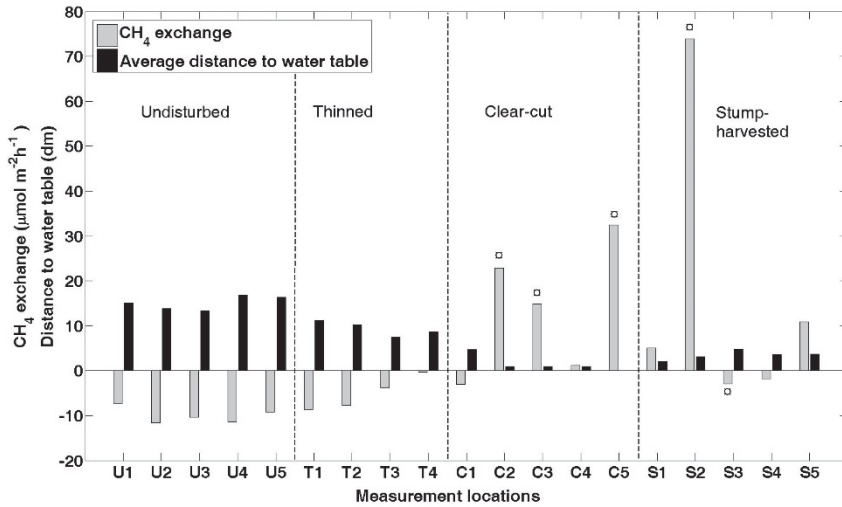
Figure 7. Fluxes of CH 4 (grey bars) from the forest floor measured with the automated chamber system in 2009-2010. The black bars represent the average distance from the soil surface to the groundwater table. The squares above the grey bars marks measurements at disturbed soil.
