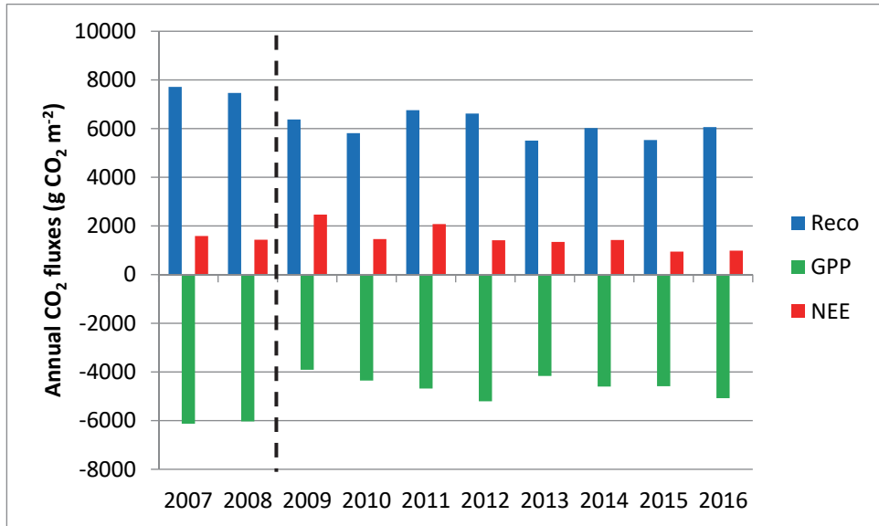
Figure 9. Annual values of net ecosystem exchange (NEE: red bars), ecosystem respiration ( R_{eco} : blue bars) and gross primary productivity (GPP: green bars) for the period 2007-2016. The vertical dashed line marks when thinning was performed.
