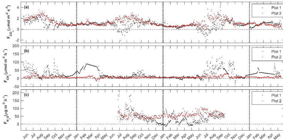
Figure 8. Daily average fluxes of \text{CO}_2 (a) and \text{CH}_4 (b) from May 2010 to May 2013 and daily average fluxes of \text{N}_2\text{O} (c) from June 2011 to September 2012. Black dots represent the wet clear-cut plot (CW) and red dots represent the dry clear-cut plot (CD). Vertical dashed lines mark the start of a new year.
