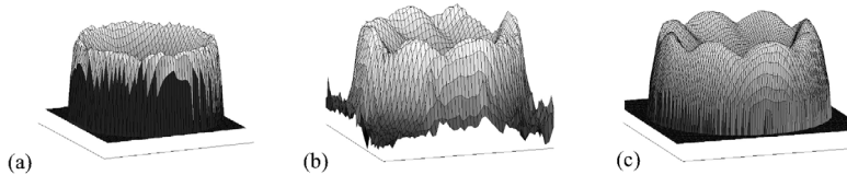
Fig. 5. The time-averaged axial velocity field at the nozzle exit from (a) the F-LES and just above of the burner from (b) the PIV measurement. The phase averaged PIV-field used as boundary condition in the G-LES are shown in (c).
