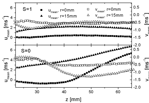
Fig. 10 Axial profiles for mean axial velocity components for swirl numbers of 0 and 1 at two radial positions as measured by PIV
