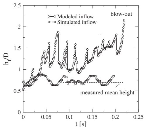
Fig. 4. Instantaneous flame front position at the axis of the burner, calculated from LES for case R20.
