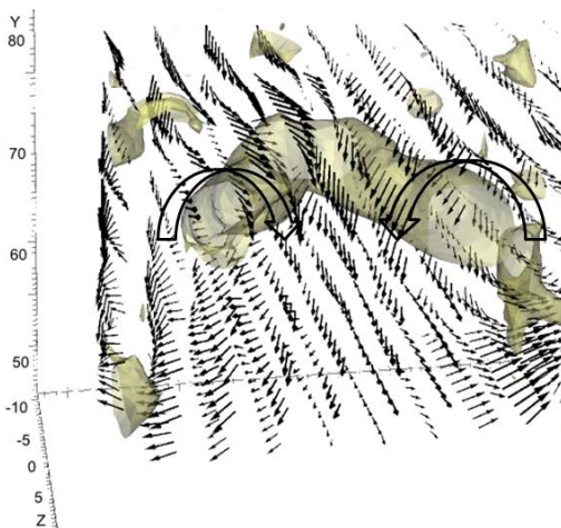
Figure 12. Instantaneous flow field and large coherent structure in the post-flame region. The iso-surfaces represent the vorticity magnitude identifying the vortex cores. The rotation direction of the vortex cores is consistent with a vortex ring.
