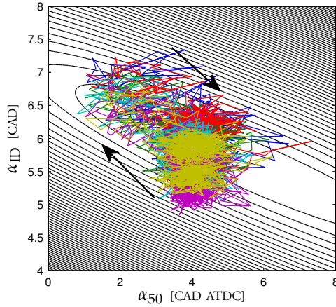
Figure 7.12 Experimental data from Fig. 7.9 illustrated in relation to cost function level curves. At engine cycle 200, the setpoint was changed from (\alpha_{50}^{\text{ref}}, \alpha_{ID}^{\text{ref}}) = (4, 5.5) to (\alpha_{50}^{\text{ref}}, \alpha_{ID}^{\text{ref}}) = (4, 6) . The arrows indicate the direction of the trajectories.
