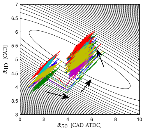
Figure 7.10 Simulation data from Fig. 7.9 illustrated in relation to cost function level curves. The setpoint is changed from (\alpha_{50}^{\text{ref}}, \alpha_{ID}^{\text{ref}}) = (2, 4.5) to (\alpha_{50}^{\text{ref}}, \alpha_{ID}^{\text{ref}}) = (5, 5) at engine cycle 200. The arrows indicate the direction of the trajectories.
