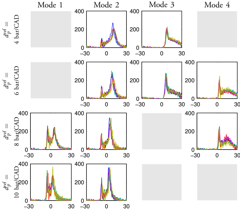
Figure 8.17 Experiments at BMEP = 4.6 bar. Heat release rates dQ [J/CAD] vs. \alpha [CAD] for Mode 1–4 (left to right), for d_p^{\text{ref}} = 4, 6, 8, 10 bar/CAD (top to bottom).
