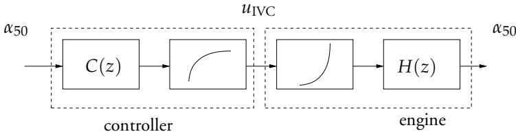
Figure 8.7 The structure of the controllers C_i where a linear controller C_{nom}(z) is combined with the inverse of the process nonlinearity to achieve an approximately linear closed-loop system.
