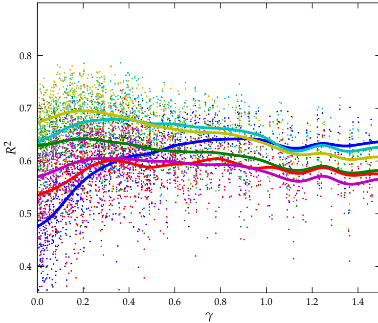
Figure 5.17 Monte-Carlo simulation where neural networks were trained for 1,000 random values of \gamma . R^2 denotes how well the cylinder- individual predicted outputs match the cylinder- averaged target output. The lines correspond to E(R_c^2|\gamma) for Cylinder c . Compared to Fig. 5.16, it can be seen that the optimal match between cylinder- individual inputs and cylinder- averaged target in this case occur for \gamma > 0 . Blue = Cyl. 1, Green = Cyl. 2, Red = Cyl. 3, Cyan = Cyl. 4, Magenta = Cyl 5, Yellow = Cyl. 6.
