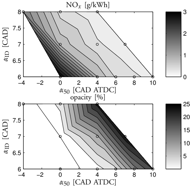
Figure 7.1 Emissions of \text{NO}_x and PM mapped according to \alpha_{50} and \alpha_{ID} for steady-state operation. Circles represent measurement points, intermediate values are obtained by linear interpolation.
