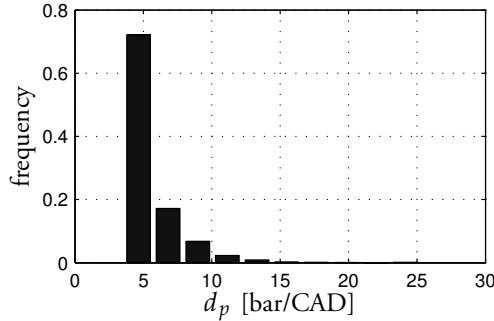
Figure 8.23 Distribution of d_p for operation at BMEP = 18.4 bar.
