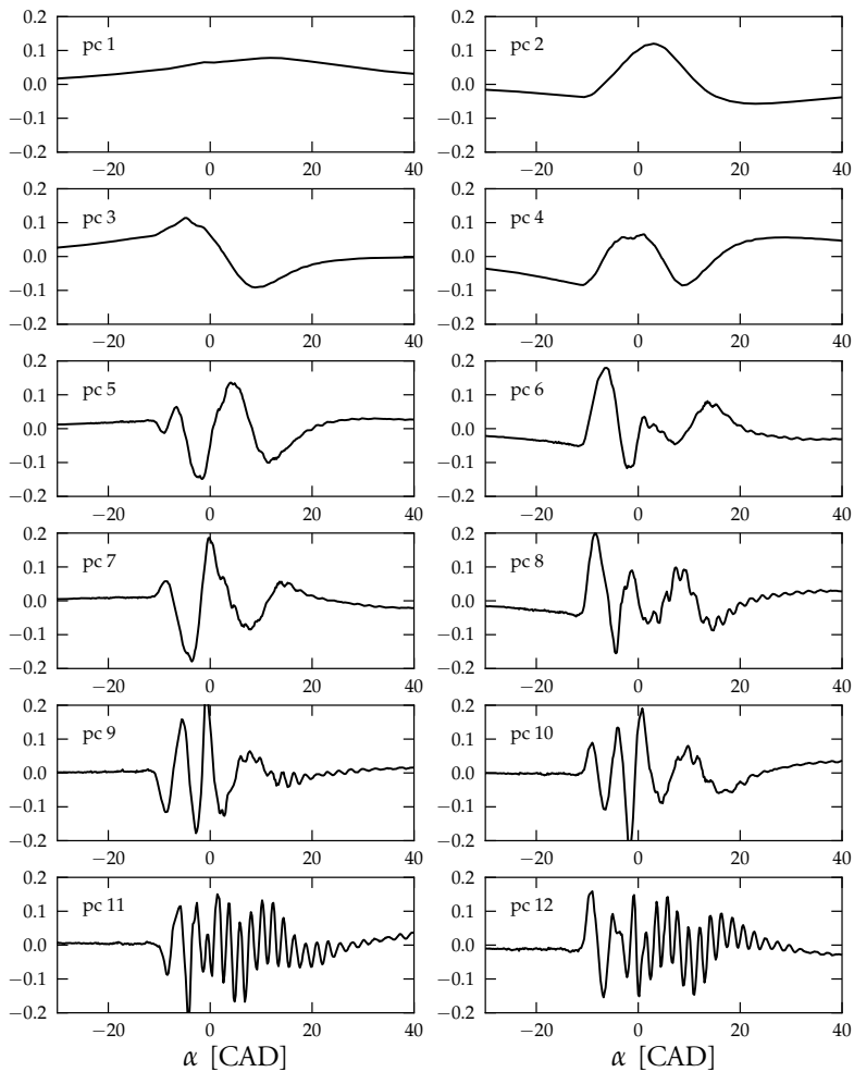
Figure 5.8 The first 12 principal components from the cylinder pressure data set.
