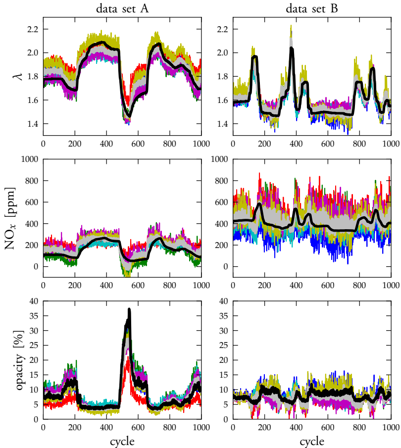
Figure 5.15 Target outputs \zeta (black), predicted output averaged over cylinders \hat{\zeta} (grey), and cylinder-individual predicted outputs (colors), for the data sets A and B.
