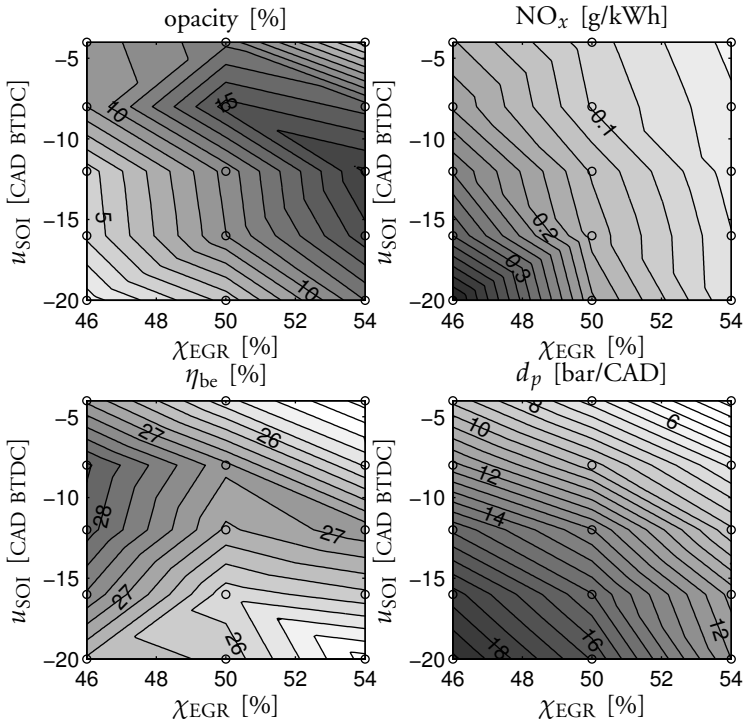
Figure 5.2 Emissions of NO_x and soot, brake efficiency \eta_{be} , and pressure derivatives d_p mapped according to u_{SOI} and \chi_{EGR} in steady-state operation. Circles represent measurement points, intermediate values are obtained by linear interpolation. All data was collected at IMEP_n = 4 bar and N_{engine} = 1200 rpm.
