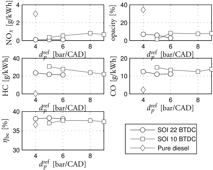
Figure 8.21 Emissions and brake efficiencies for experiments at BMEP = 9.2 bar.
