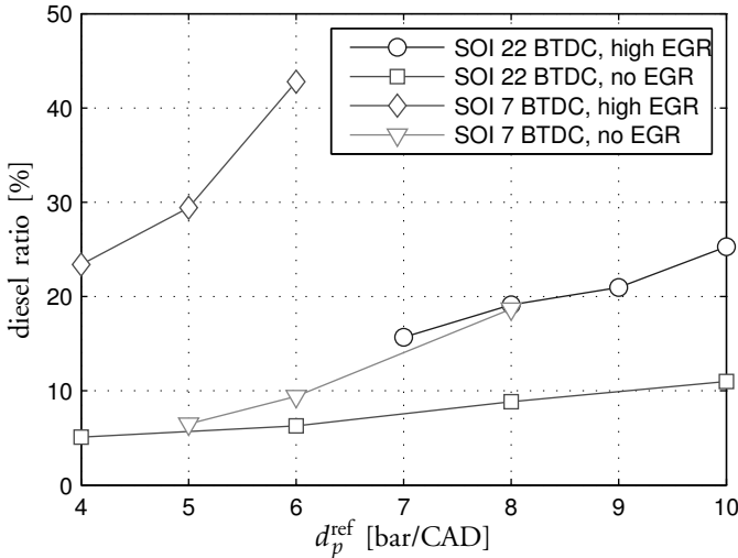
Figure 8.16 Ratio of diesel energy to total fuel energy required to keep a certain d_p for the four operation modes tested at BMEP = 4.6 bar. With pure diesel operation without EGR, average d_p was 5.4 bar/CAD.
