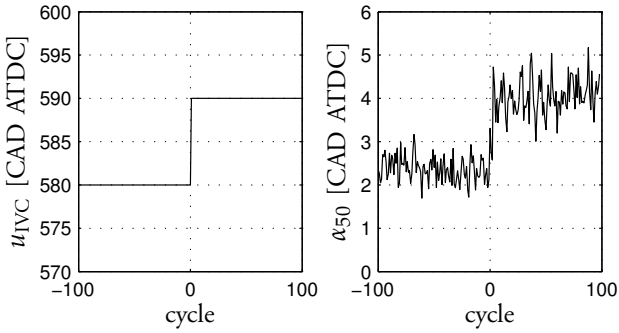
Figure 8.2 Step response from u_{IVC} to \alpha_{50} .
