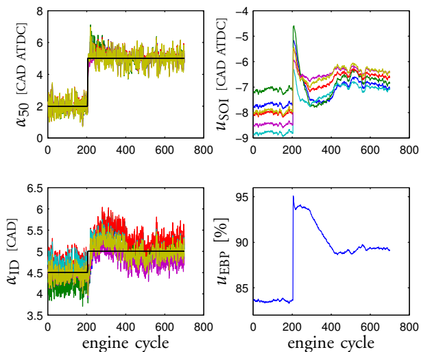
Figure 7.9 Simulation results using the decentralized controller. At engine cycle 200, the setpoint is changed to the cost function optimum.
