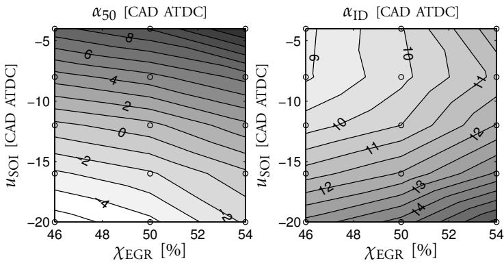
Figure 5.3 Feedback variables \alpha_{50} and \alpha_{ID} mapped according to u_{SOI} and \chi_{EGR} for steady-state operation.
