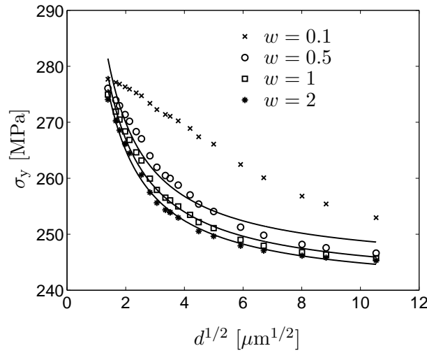
Figure 10: Variation of the flow stress, obtained at \varepsilon_{\text{eff}}^{\text{P}} = 0.25 , for different grain sizes and for different values of the w -parameter, corresponding to the values used in Fig. 8. Symbols represent simulation results and solid lines least-squares fittings of the Hall-Petch relation in eq. (11).
