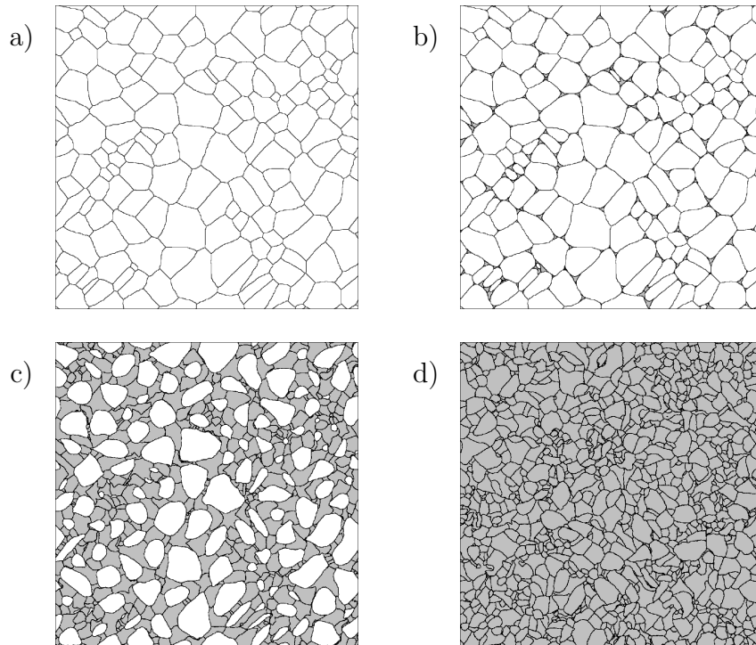
Figure 13: Microstructure at different deformation states, cf. Fig. 11a. Recrystallized grains are shaded gray. a) Initial microstructure with 150 grains and an average grain size of 45 \mu\text{m} at \varepsilon_{\text{eff}}^{\text{p}} = 0 , b) Growth of the first nuclei from triple junctions at \varepsilon_{\text{eff}}^{\text{p}} = 0.56 , c) Necklace pattern of recrystallized grains at \varepsilon_{\text{eff}}^{\text{p}} = 0.63 and d) Final grain structure with 977 grains and an average grain size of 16 \mu\text{m} at \varepsilon_{\text{eff}}^{\text{p}} = 2 .
