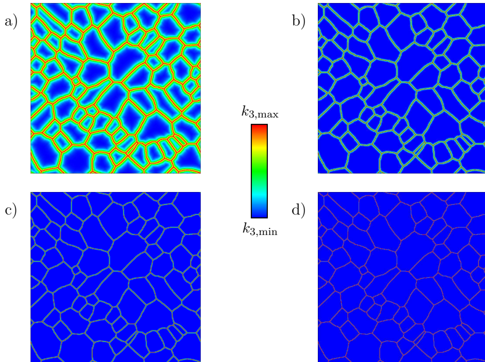
Figure 8: Variation of the k_3 parameter in a 2D microstructure with 75 grains and an average grain size of d = 64 \mu\text{m} . The different figures are obtained by different choices of the parameter w : a) w = 0.1 , b) w = 0.5 , c) w = 1 and d) w = 2 .
