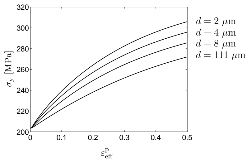
Figure 9: Homogenized flow stress obtained from the polycrystal simulations for some different grain sizes and with w = 0.1 .
