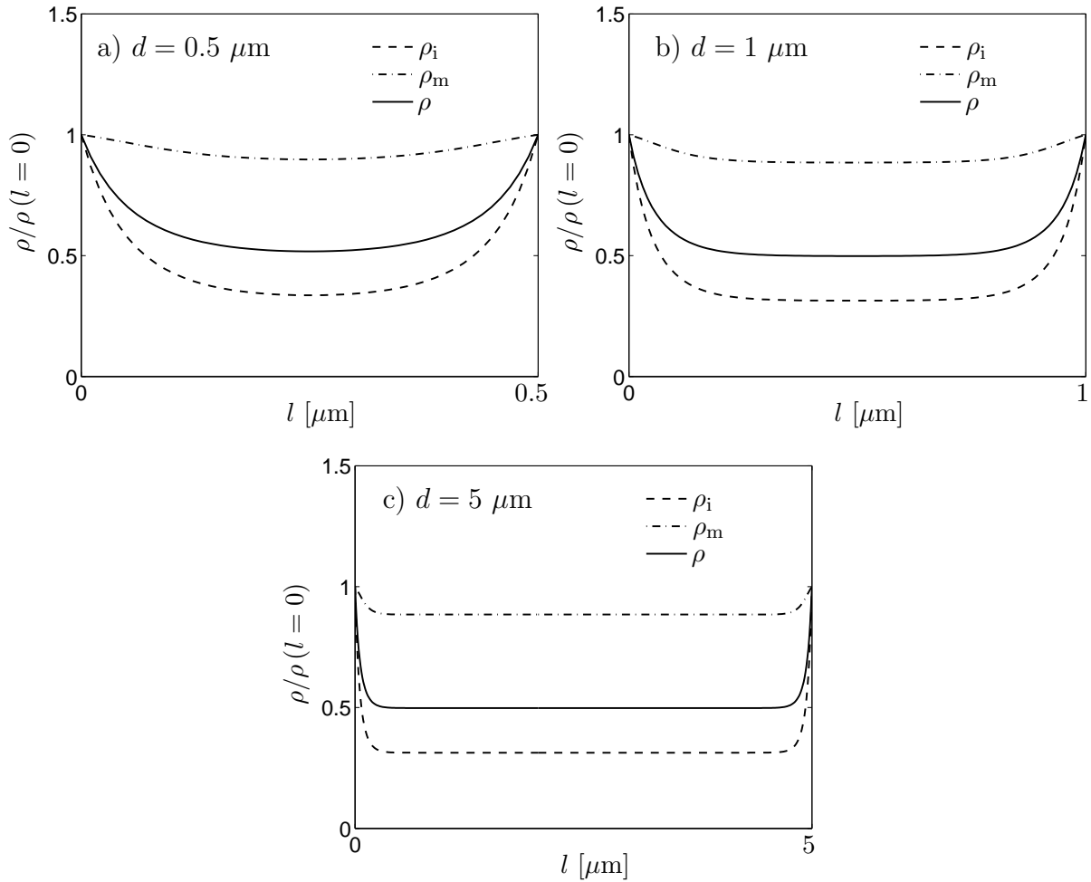
Figure 2: Distribution of dislocation density in grains of different diameter d at an effective plastic strain of \varepsilon_{\text{eff}}^p = 0.5 . Note that the individual dislocation densities are normalized by their values at l = 0 : a) d = 0.5 \mu\text{m} , b) d = 1 \mu\text{m} and c) d = 5 \mu\text{m} .
