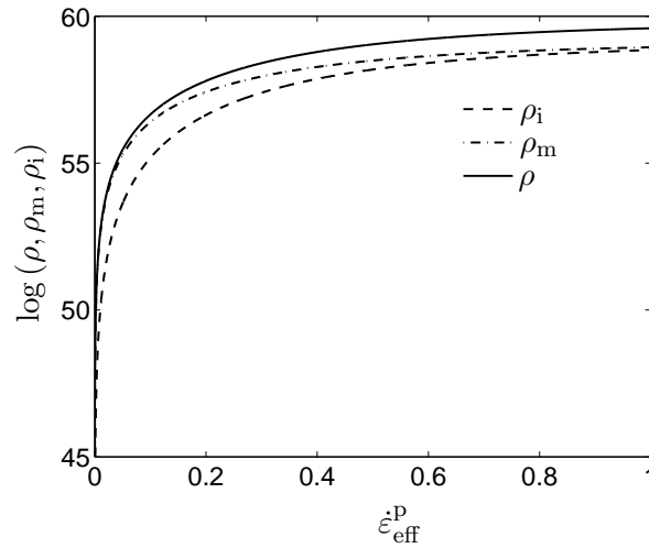
Figure 3: Average dislocation densities in a one-dimensional grain with diameter d = 1 \mu\text{m} as functions of macroscopic effective plastic strain.
