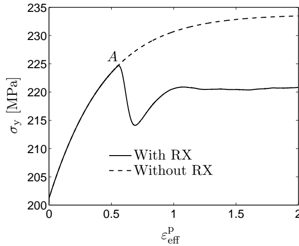
Figure 11: Flow stress behavior obtained from the cellular automaton simulation. The onset of recrystallization occurs at point A. Results from a simulation with recrystallization (RX) is shown by a solid line and results without recrystallization is shown by a dashed line.
