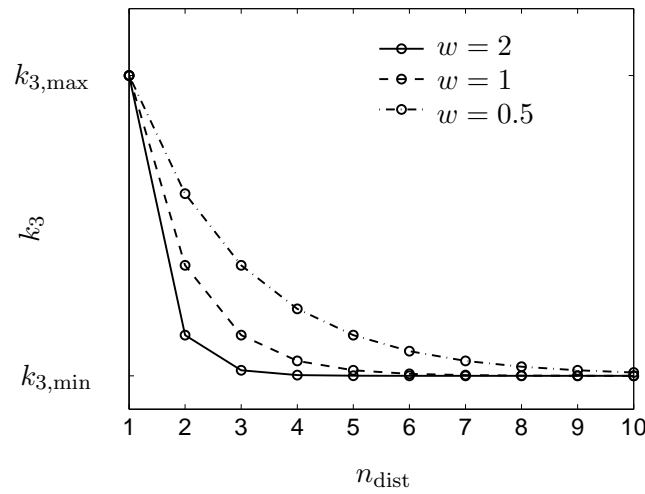
Figure 6: Variation of the k_3 -parameter within a grain in the computational cell grid using the distance numbers n_{\text{dist}} . Note that the lines are only shown to indicate the trends since in the cell grid, each value of n_{\text{dist}} represents an individual cell in which k_3 attains a constant value.
