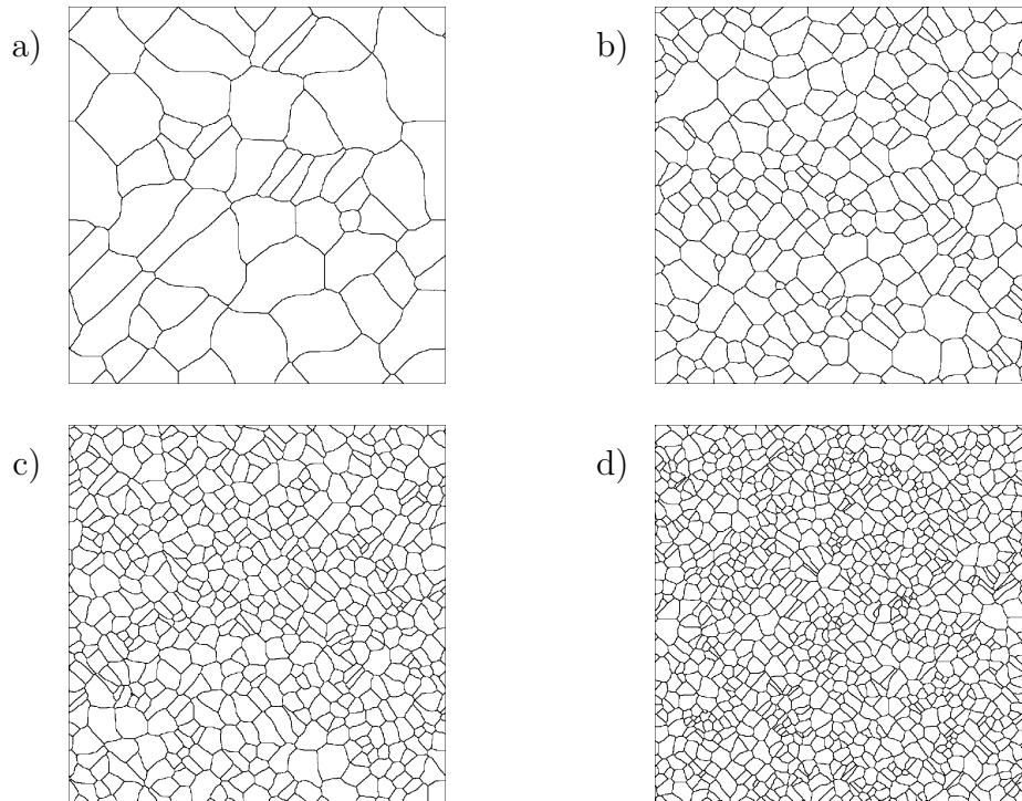
Figure 7: Examples of the microstructures used in the present simulations. The microstructures have different average grain size: a) 78 \mu\text{m} (50 grains), b) 35 \mu\text{m} (250 grains), c) 25 \mu\text{m} (500 grains) and d) 18 \mu\text{m} (1000 grains).
