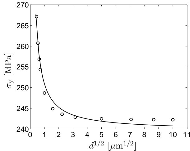
Figure 4: Variation of the macroscopic yield stress with the square-root of the grain size d^{1/2} . Results obtained from one-dimensional calculations at \varepsilon_{\text{eff}}^{\text{p}} = 0.25 , and using eq. (12), are shown as symbols and the solid line shows the fitted Hall-Petch relation in eq. (11).
