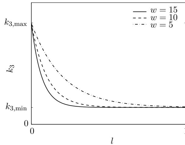
Figure 1: Variation of the k_3 parameter from the grain boundary, where l = 0 , towards the grain center. The different lines show the effect of varying the parameter w in eq. (9).
