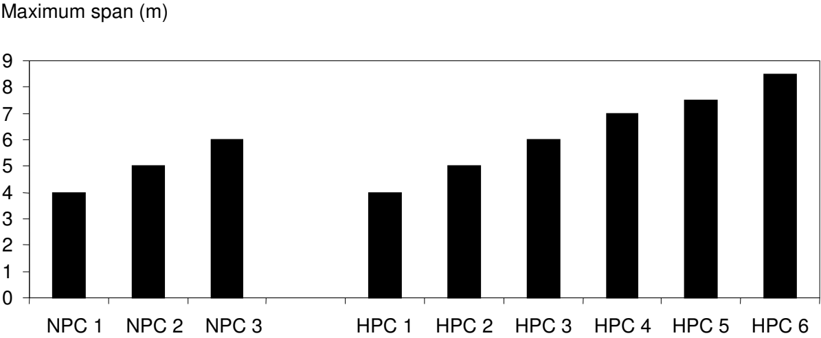
Figure A.9 Effects of various concrete and slab parameters on maximum slab span. Slab type 1.
