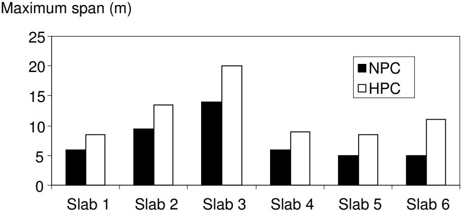
Figure A.8. Comparison between normal house-building concrete (NPC) and high performance concrete (HPC) with regard to maximum slab span allowed in all studied slab types.
