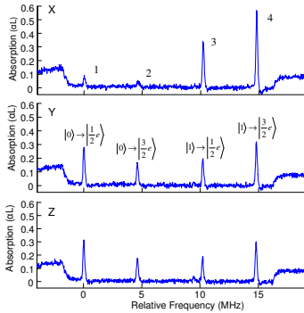
Figure 5.9. The three different projection measurements included in the quantum state tomography sequence of the state displayed in Figure 5.8. The four main peaks correspond to the qubit states' transitions to the two strongest excited states, as indicated in the Y-measurement figure.
