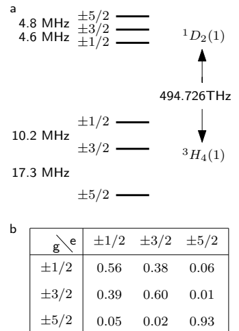
Figure 3.3. Properties for \text{Pr}^{3+}:\text{Y}_2\text{SiO}_5 . In a the level structure of \text{Pr}^{3+} is shown and b contains the relative oscillator strengths for all 9 possible transitions.
