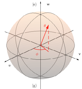
Figure 2.2. The Bloch sphere with a vector inscribed that demonstrates the two characterizing angles, \theta , and \phi .
