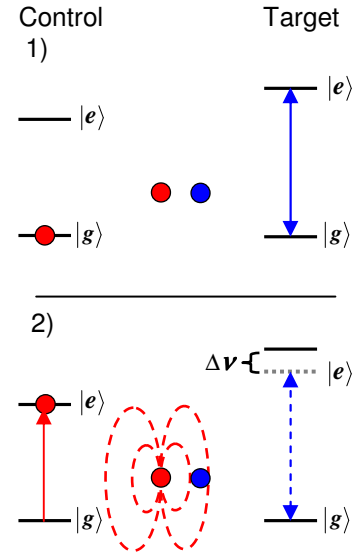
Figure 5.12. Two near-lying ions with different resonance frequencies are selected. With the control ion still in the ground state, the target ion can be involved in operations, using a frequency \nu_{ge} . In part 2), the control ion is excited and due to the Stark shift from the changed dipole moment, the target ion is no longer accessible as frequency \nu_{ge} .
