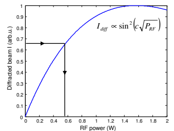
Figure 4.5. Graph showing the intensity in the diffracted beam as a function of RF power. The arrows illustrate that a function is needed to find the RF power for any pulse intensity value.
