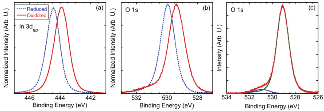
FIG. 9. (Color online) PES on the sputtered/annealed (reduced) and oxidized samples of the (a) In 3d_{5/2} and (b) O 1s core levels, taken with a photon energy of 610 eV. (c) Line fits of the O 1s peak of the oxidized surface at 610 eV.
