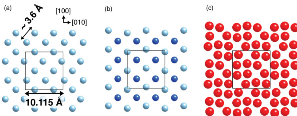
FIG. 10. (Color online) Models of the In 2 O 3 (001) surfaces with (a) D-layer, (b) M-layer (b), and (c) O-layer termination. Shown are bulk-terminated layers with all the indium and oxygen atoms present; In-b atoms are shown darker than In-b. Note that these terminations represent polar surfaces; for stoichiometric surfaces, only half of the atoms shown here are expected to be present.
