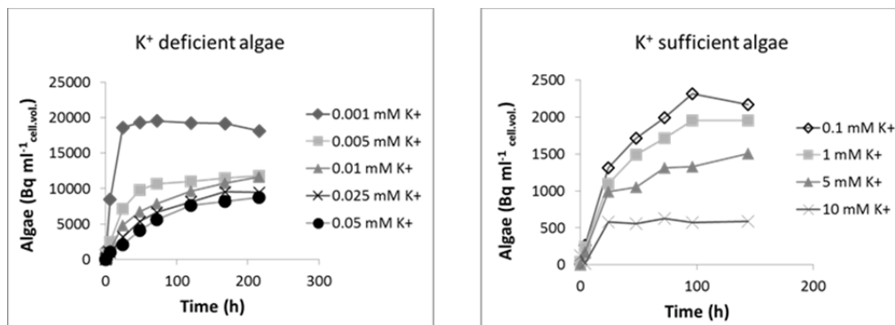
Figure 1. Time course of ^{137}Cs uptake by K^+ deficient and K^+ sufficient microalgae in K^+ supplemented cultures (1 \mu M K^+ and 0.1 mM K^+ are the control cultures for deficiency and sufficiency; data are the mean of 3 replicates)
