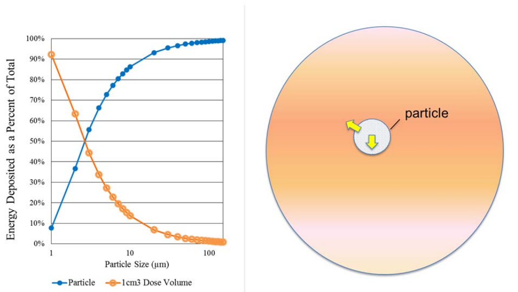
Figure 8. MCNP6 model data indicating percentage of alpha emission energy that is deposited within a Pu-containing particle (blue symbols), vs that deposited in surrounding tissue (orange symbols) (adapted from Caffrey et al., 2016)
