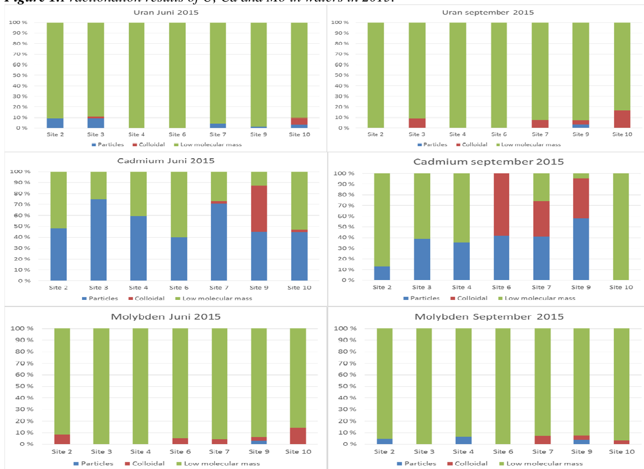
Figure 1. Fractionation results of U, Cd and Mo in waters in 2015.
