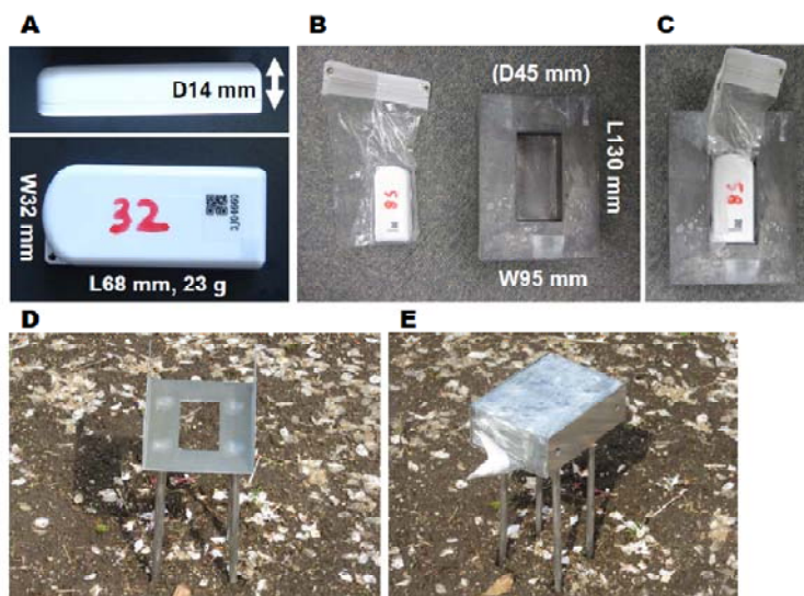
Figure 1. Measurement apparatus and settings
