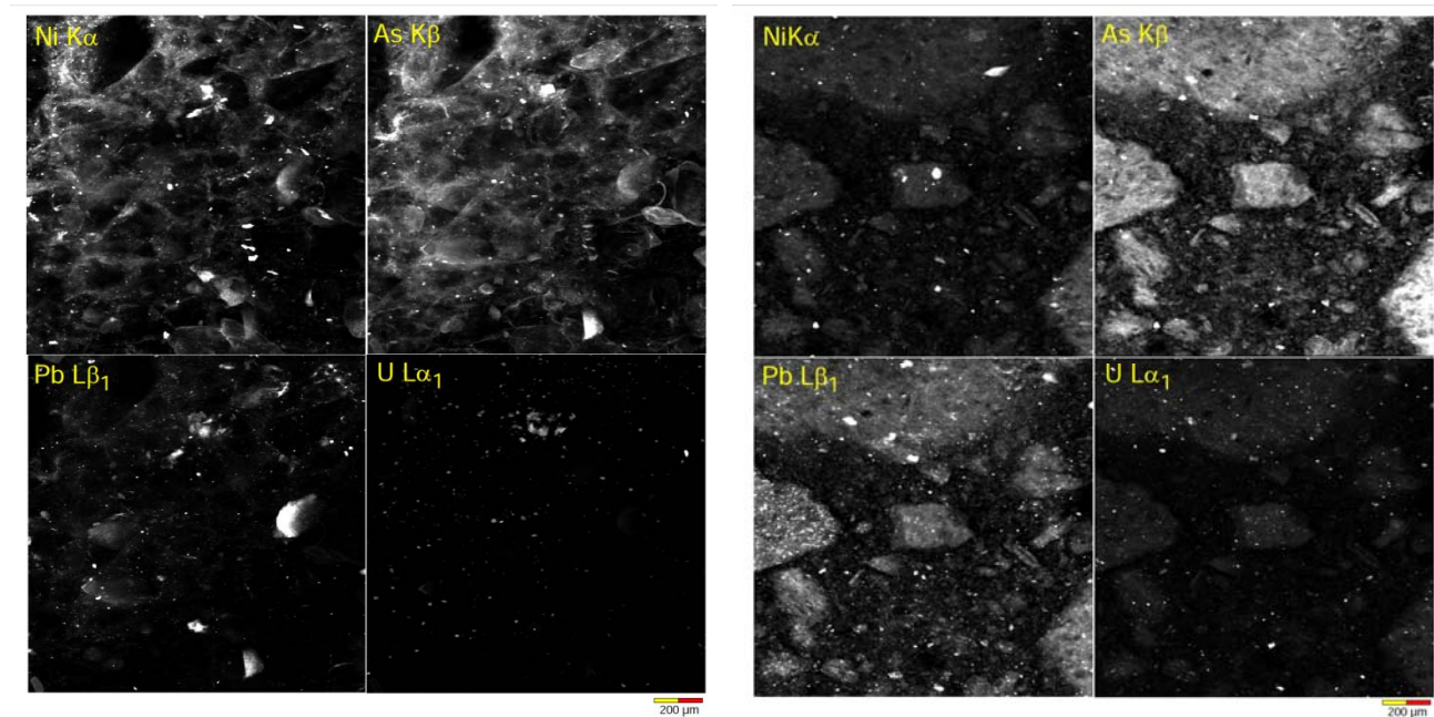
Figure 2. X-ray fluorescence intensities from 1.5 x 1.5 mm compositional maps of section TMF02-SA05-Map4 (left panel, 400 masl) and TMF01-SA19-Map2 (right panel, 369 masl). Maps show Ni K\alpha , As K\beta , Pb L\beta_1 and U L\alpha_1 separately. All are displayed as two dimensional grayscale with white being the highest intensity, 40 msec accumulation time per 2 \mu\text{m} pixel.
