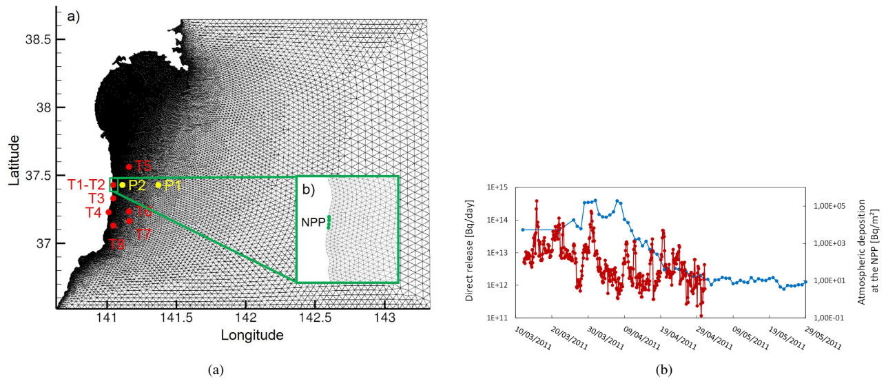
Fig. 2: a) Computational grid and sampling points where calculated ^{137}\text{C}_s concentrations in surface water have been compared with measurements. Points P1 and P2 are issued from the MODARIA project Exercise 1. The grid points employed for reproducing the NPP are indicated in green; b) Source term of caesium ^{137}\text{C}_s used in the numerical simulations, see section -B.
