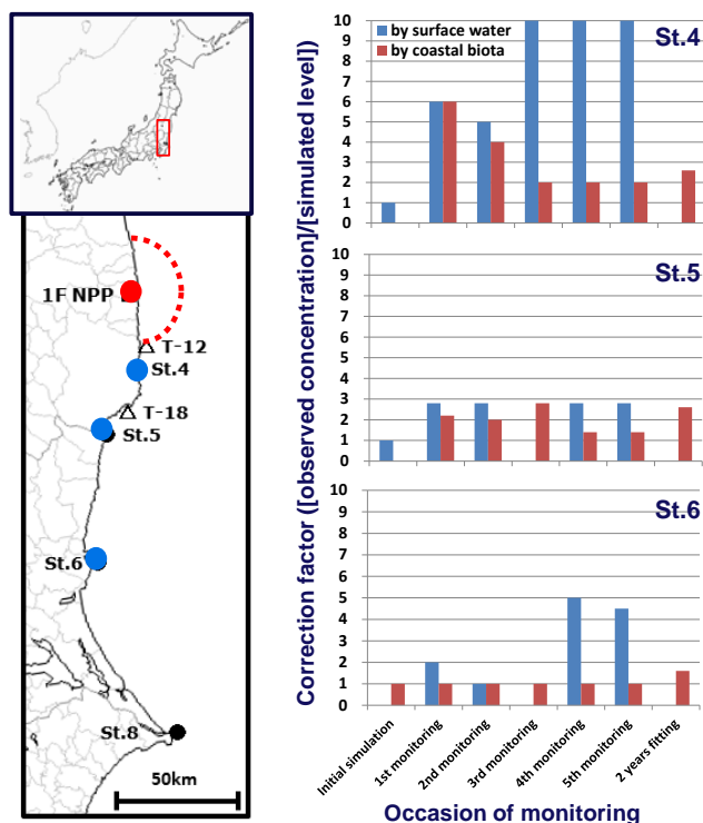
Figure 3. Correction factors derived by seawater (blue bar) and bio-monitor (red bar) in each occasion at southern coastal area (St. 4 to 6) during 7 th April, 21 st April, 6 th May, 2 nd June, 16 th July 2011.
