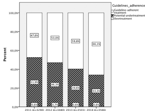
Fig. 1. Guideline adherence 2011–2014.
