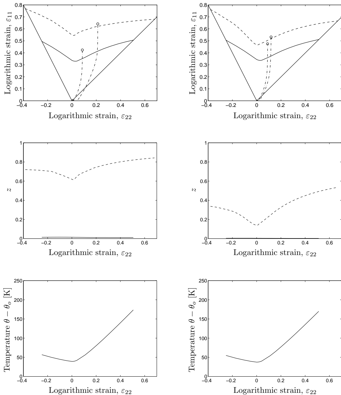
Figure 7: Fig. 6 continued. The left and right columns represent analysis with an initial temperature of 293 K and 313 K, respectively.
