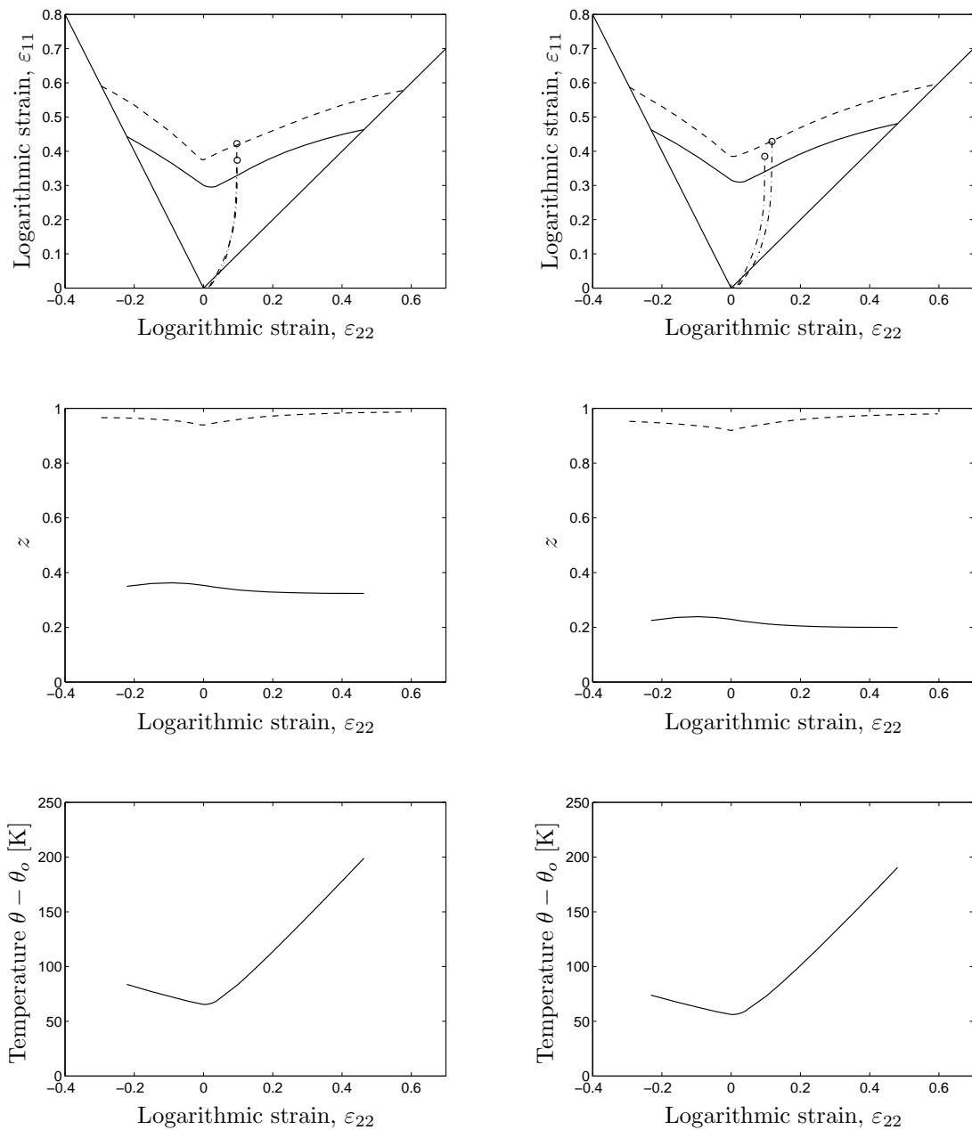
Figure 6: The left and right columns represents analyses with an initial temperature of 213 K and 233 K, respectively. The figures in the top row are the forming limit diagrams. The figures in the middle row shows the fraction of martensite at the onset of shear band formation and the bottom row figures show the temperature change at shear band initiation. Solid lines represent results from adiabatic simulations and dashed lines correspond to isothermal simulations. Similar results for the initial temperatures 293 K and 313 K are shown in Fig. 7. Dash-dotted lines show the strain paths traced in the localization region of the plate during the simulations of cup deep-drawing processes, also considered in the present work.
