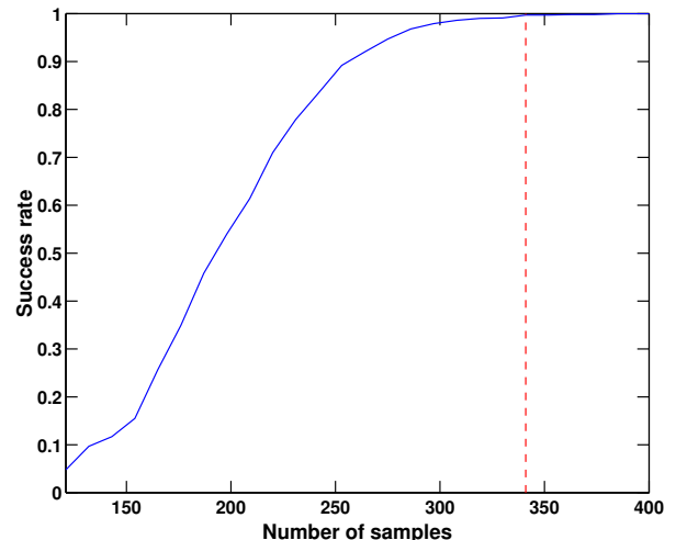
Fig. 5. Rate of success for PECS G in estimating the periodicities of a signal with periodicities at 11 and 31, as a function of signal length. The dashed line denotes the minimum data needed for using [8].
