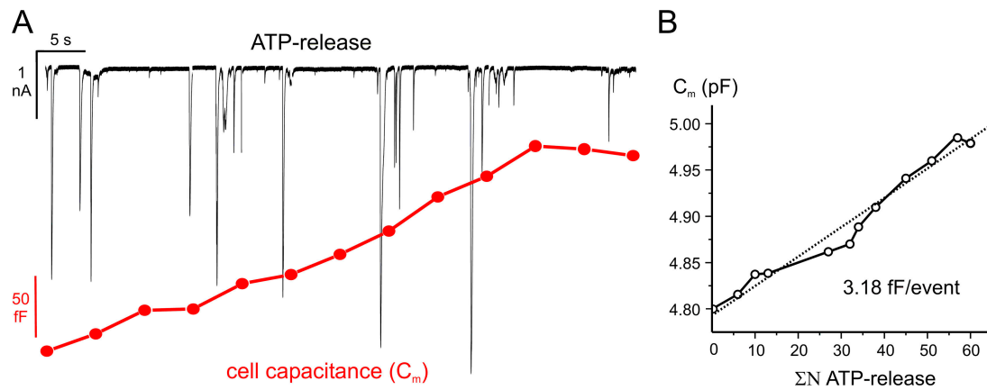
Figure 2. Estimation of the unitary LDCV capacitance increase. (A) P_2X_2 receptor-mediated TICs (top) and increase in whole-cell capacitance (bottom) recorded simultaneously in the same cell. Exocytosis was elicited by inclusion of 230 nM free Ca^{2+} in the pipette solution. Each segment (5 s) was preceded by a brief prepulse with a sine wave to measure the cell capacitance. (B) Plot of the cumulative number ( \Sigma N ) of purinergic TICs vs. membrane capacitance ( C_m ) from the same experiment. A linear fit (dotted line) with a slope of 3.18 fF/event is superimposed.
