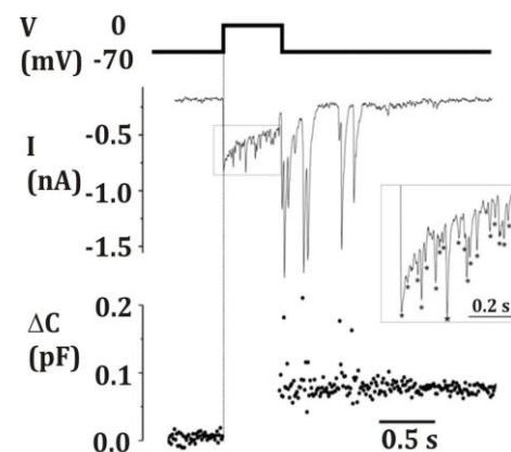
Figure 10. Time course of nucleotide release. The 500 \text{ ms} depolarization pulse to 0 \text{ mV} (above), ATP currents (middle) and cell capacitance recording (below). The inset shows the expanded indicated part (highlighted by square). Asterisks indicate current spikes superimposed on the inward \text{Ca}^{2+} -current (identified by eye).
