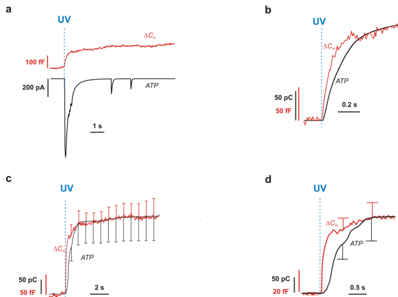
Fig. 5. Time course of ATP release and association with capacitance increase. a Predicted time course of ATP release (black trace) following photorelease of caged \text{Ca}^{2+} based on a capacitance increase of 130 fF with a t_{1/2} of 55 ms (red trace). b Comparison of time courses of capacitance increase (red trace) and cumulative TIC charge for modelled ATP trace in panel a. c Cumulative charge of TICs of the five cells shown in Fig. 4a-b (black) superimposed on the mean capacitance increase in untransfected cells (red). For clarity, error bars (S.E.M.) are only shown for every 20 (capacitance) and 3500 (charge) points. d Same data as in c but the first 2 s shown on an expanded time bases.
