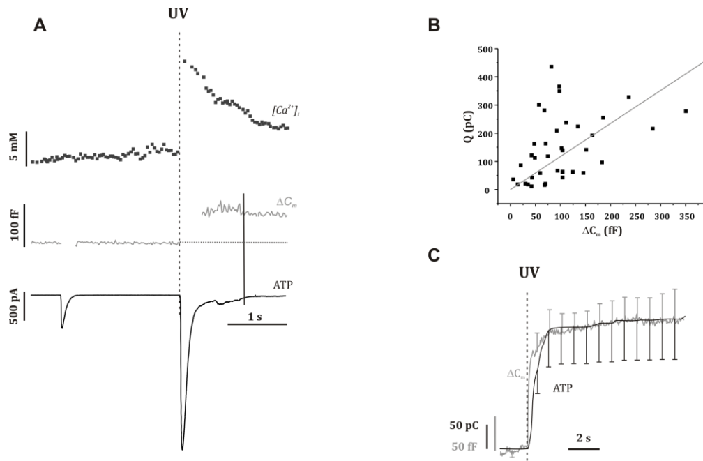
Figure 24. P2X 2 receptor currents and changes in \beta -cell membrane capacitance evoked by photorelease of caged Ca^{2+} . (A) Increase in [Ca^{2+}]_i (top), change in membrane capacitance (middle) and associated P2X 2 R currents (bottom) transients recorded from a rat \beta -cell. (B) Relationship between capacitance increase ( \Delta C_m ) and total TIC charge ( Q ) evoked by photorelease of caged Ca^{2+} . A straight line was fitted to the data points with a slope of 1.2 \pm 0.2 pC/fF ( r=0.8 ; P<0.001 ). The charge and capacitance was measured over the period indicated by dashed vertical line in (A). (C) Cumulative charge of TICs (black; n=6 ) superimposed on the mean capacitance increase in untransfected cells (grey; n=5 ).
