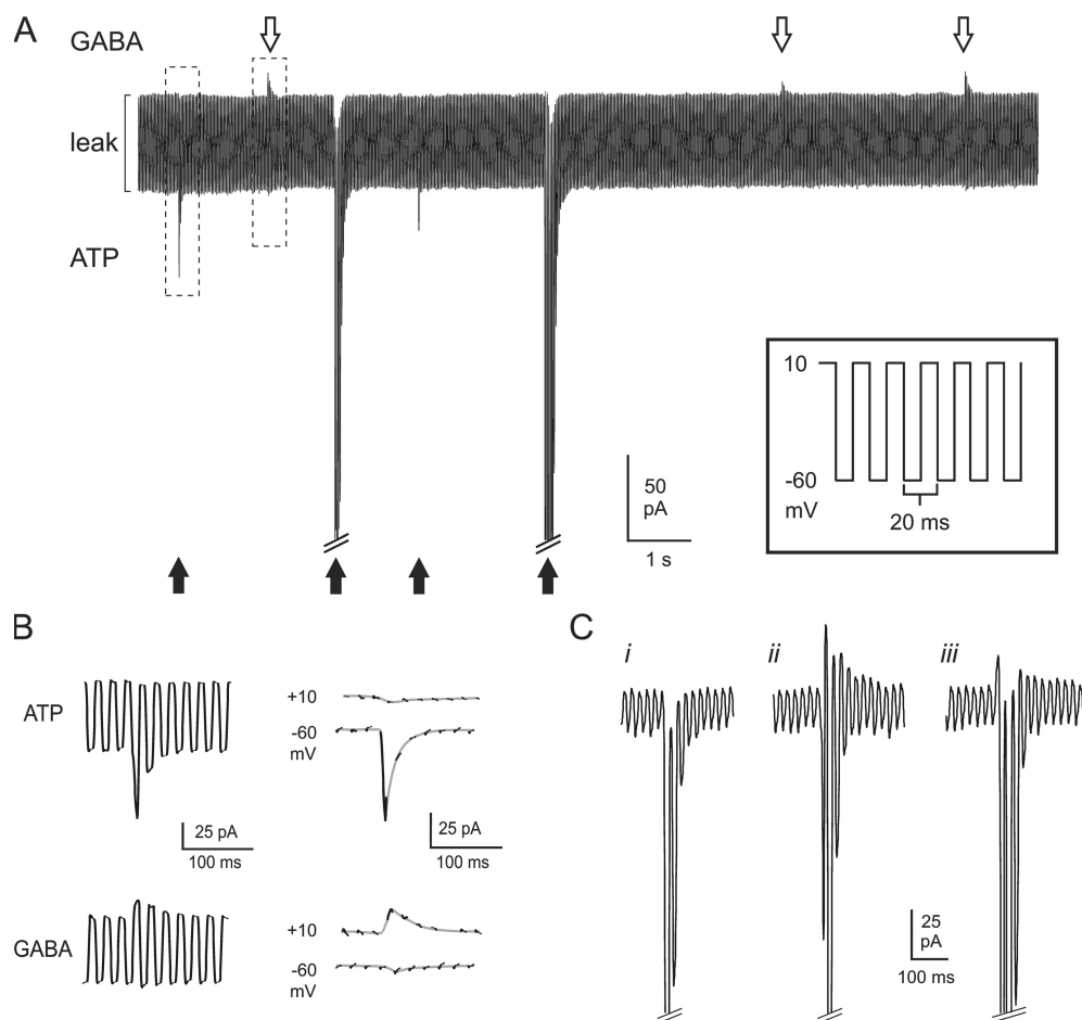
spective voltages have been connected by gray lines. (C) Examples of different types of events with a dominant inward current component: (i) inward current in isolation; (ii) clear out- and inward components; (iii) an outward component superseded by the activation of the inward current. The inward currents at -60 mV have been truncated for display purposes.
