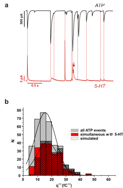
Fig. 3. P2X 2 R currents associated with serotonin release. a Examples of amperometric events (red) with parallel recordings of TICs (black). Red lines indicate simultaneous events. A single amperometric event not associated with a detectable TICs has been highlighted by the arrow. b Distribution of ^3\sqrt{q} of all events (grey) and the events associated with serotonin release (red) when exocytosis was evoked by 0.2 \mu\text{M} [\text{Ca}^{2+}]_i and 100 \mu\text{M} cAMP. The stippled bars represent the distribution obtained from the original one (grey bars) when allowance is made for the diffusion of ATP and assuming detection of the ATP-dependent TICs been by an amperometric sensor (cf. [12]).
