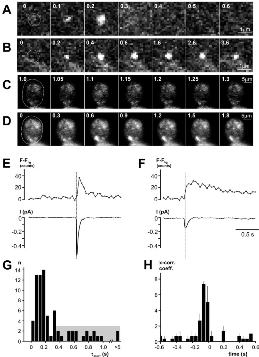
Fig. 6. Parallel recording of nucleotide and peptide release from individual granules. (A,B) Confocal images of a section of the footprint of a voltage-clamped cell expressing both IAPP-pHluorin and P2X 2 -mRFP. The images were recorded at the indicated times relative to the onset of the IAPP-pHluorin flash. Exocytosis was elicited by intracellular dialysis of the cell with a buffer in which [Ca^{2+}]_i was set at 2 μM. Note that the highlighted granules increase their fluorescence during the displayed sequence. In A, the signal from the granule is rapidly lost, while in B it remains elevated for several seconds. (C,D) Image sequences of a cell co-transfected with IAPP-pHluorin and P2X 2 -mRFP1 and stimulated as in A and B. The entire cell was imaged in the IAPP-pHluorin channel (see Materials and Methods), and whole-cell current spikes due to activation of the P2X 2 receptors were recorded in parallel. Examples of a short-lived fluorescence transient in C, and a long-lasting event in D. (E,F) Time course of the average fluorescence intensity in the ROIs indicated by the white circle in C and D (top) and inward membrane currents associated with the events (lower). Note slow decay of fluorescence in F. (G) Histogram of the decay constants of 56 events as in C and D. The shaded area indicates decay constants greater than 350 milliseconds. (H) Cross-correlation histogram of the times of fluorescence peaks vs the times of current peaks in three experiments similar to that shown in C and D.
