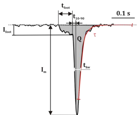
Figure 8. Definition of parameters often used in the analysis of ATP current spikes. Spike baseline – dashed line, I_m – spike amplitude; Q – overall charge moved into the cell by the current spike equal to the integral of current over the duration of the spike; t_{10-90\%} – 10 to 90% rise time; t_{hw} – the halfwidth of the spike measured at 50% of I_m ; \tau – the decay time of the spike measured between 75% of I_m and baseline; I_{foot} – the foot current amplitude; t_{foot} – foot duration.
