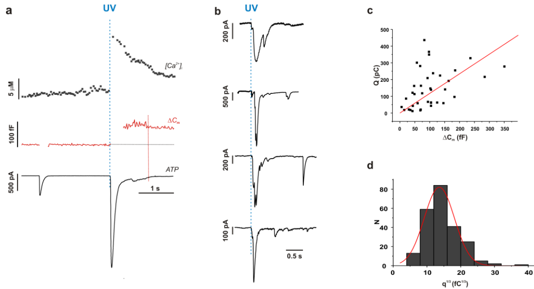
Fig. 4. P2X 2 receptor currents and changes in \beta -cell membrane capacitance evoked by photorelease of caged Ca^{2+} . a Increase in [Ca^{2+}]_i (top), change in membrane capacitance (middle) and associated P2X 2 R currents (bottom) transients recorded from a rat \beta -cell. The capacitance measurements are not shown during the period associated with the TIC to remove large artefactual transients. b Examples of TIC responses following photorelease of Ca^{2+} in another 4 cells. c Relationship between capacitance increase ( \Delta C_m ) and total TIC charge ( Q ) evoked by photorelease of caged Ca^{2+} . A straight line was fitted to the data points with a slope of 1.2 \pm 0.2 pC/fF ( r=0.8 ; P<0.001 ). The charge and capacitance was measured over the period indicated by dashed vertical line in (a). d Distribution of spontaneous events observed prior to photorelease of [Ca^{2+}]_i . A Gaussian has been superimposed.
