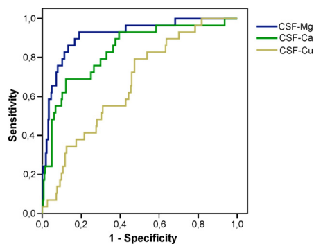
Fig. 3. Receiver operating characteristic (ROC) curves of CSF-Mg, CSF-Ca and CSF-Cu for differentiation of DLB patients from all patients with Alzheimer's disease (AD) and AD. The areas under the ROC curve for the analyzed metals with 95% confidence interval were: CSF-Mg, 0.92 (0.86–0.97), CSF-Ca 0.84 (0.76–0.92) and CSF-Cu 0.66 (0.57–0.76), respectively.
