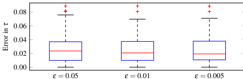
Figure 9. Boxplots of the absolute errors in the estimation of \tau , for the three different convergence limits \epsilon = \{0.05, 0.01, 0.005\} .
