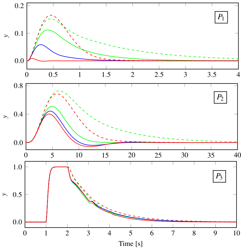
Figure 7. Step responses from a load disturbance on the process input, shown for the closed-loop systems containing the true processes and the different obtained controllers. The green curves show controllers tuned for the ITD/FOTD models, blue shows controllers tuned for IFOTD/SOTD models, red shows controllers tuned for the true processes. The dashed lines indicate the PI controllers, while the solid lines show the PID controllers.
