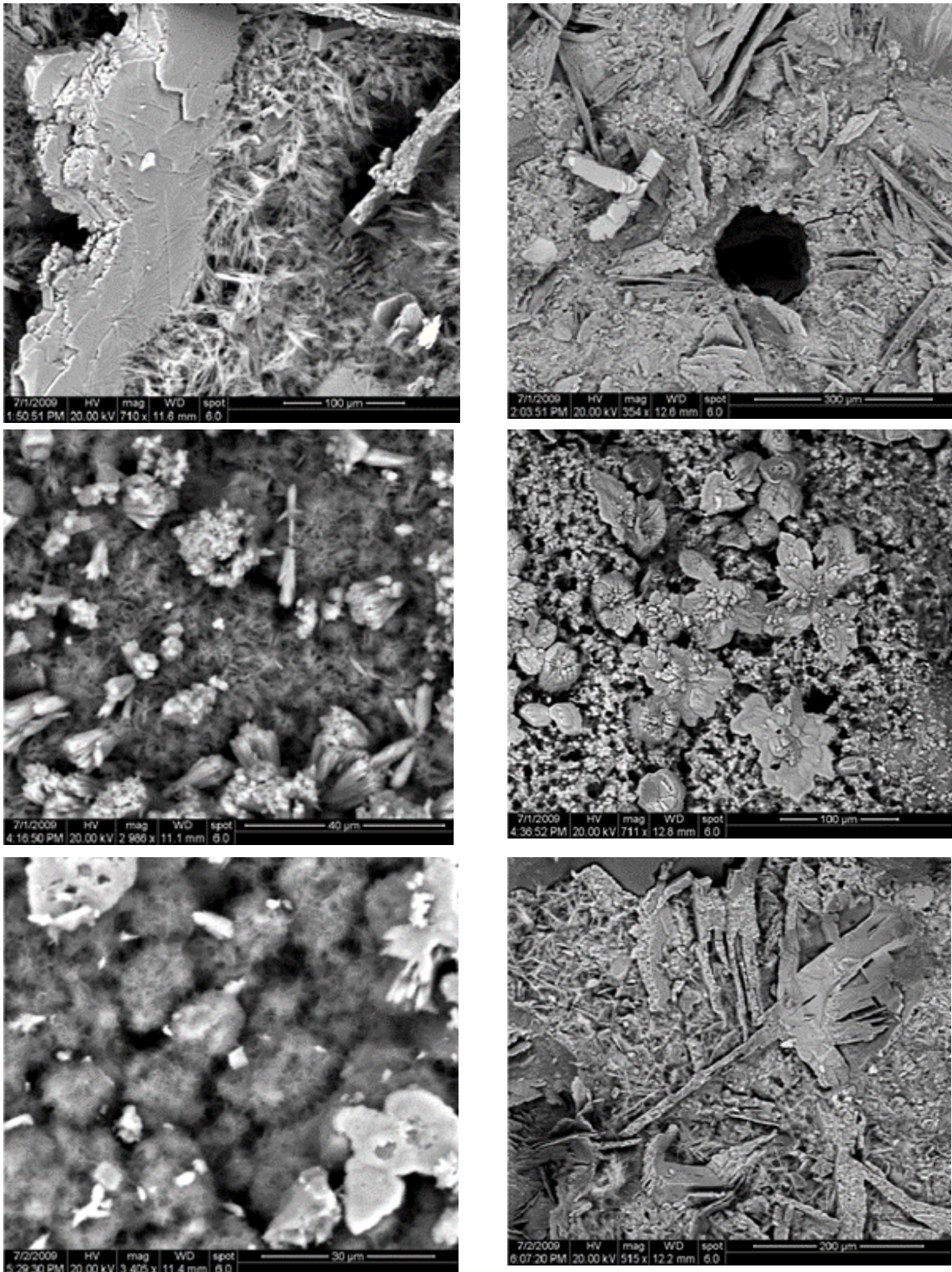
Figure 14.5: SEM-photos of precipitations in cracks for specimens exposed to cyclic immersion in sea water and drying. Photos: Kalinowski & Fjällberg (2010). Upper row: Cover 55 mm. Crack 0.2 mm. Specimen H55-2-2-1. Left: Depth 25 mm. Right: Depth 55 mm. Middle row: Cover 55 mm, Crack 0.4 mm. Specimen H55-4-2-1. Left: Depth 5 mm. Right: Depth 55 mm. Lower row: Cover 55 mm. Crack 0.4 mm. Specimen H55-4R-2-1. Relaxed crack Left: Depth 5 mm. Right: Depth 55 mm.
