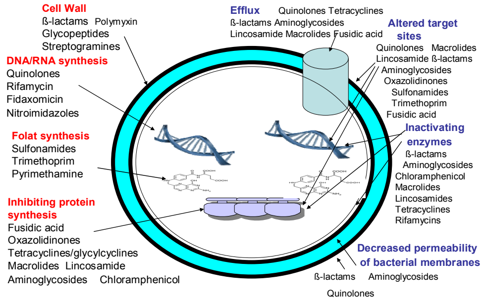
Figure 1: Mechanisms of antimicrobial activity and of antibiotic resistance
