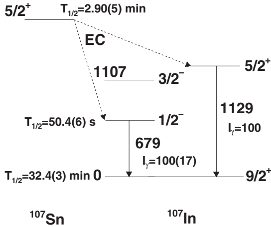
FIG. 2. Partial level scheme of ^{107}\text{In} , indicating the electron capture (EC) decay of ^{107}\text{Sn} . The energies are given in keV. The two indicated \gamma -ray transitions were used to estimate the ^{107}\text{In}^m contamination. The data were taken from Ref. [24].
