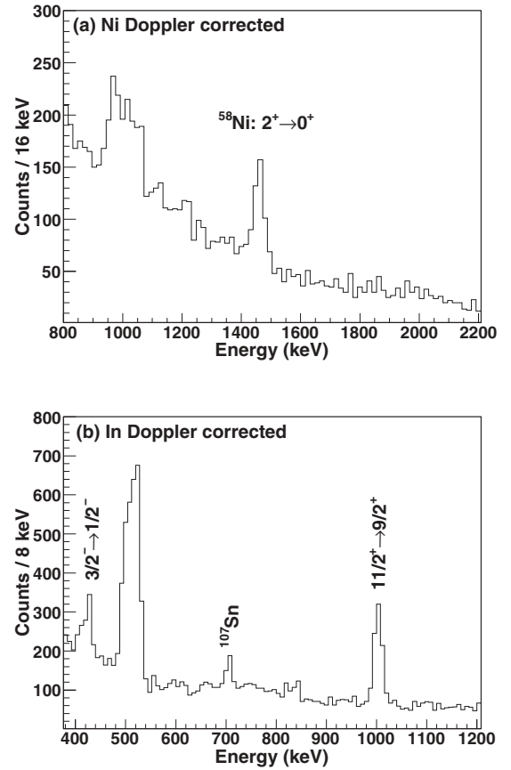
FIG. 1. The \gamma -ray spectra from the experiment, using either (a) Ni or (b) In particles for Doppler correction. The structure around 500\text{ keV} results from the 511\text{ keV} line, which collapses during the Doppler correction.
