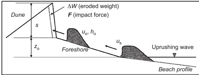
Figure 1. Definition sketch for analytical model of dune erosion
