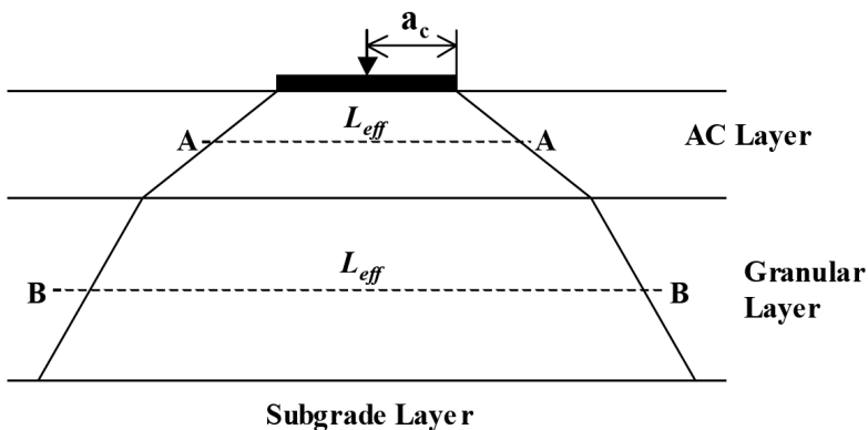
Figure 3-6. Effective length approximation in each sublayer (NCHRP, 2004).
