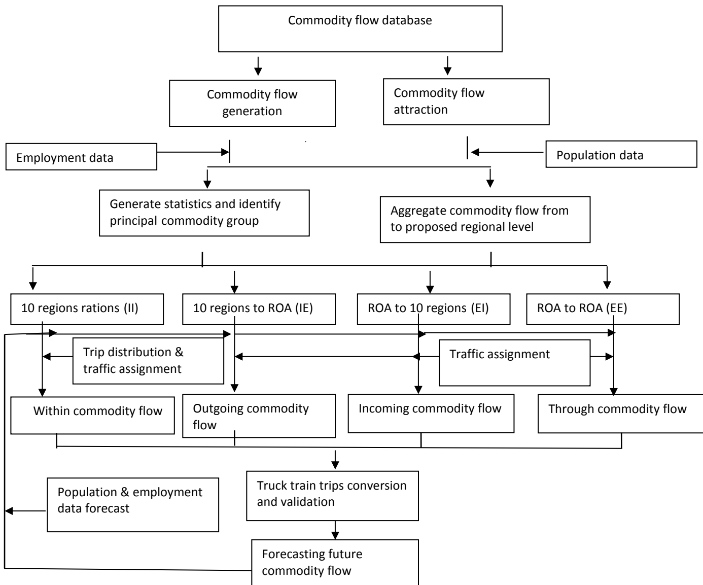
Figure 4.3: Structured analysis procedures for transportation analysis Note: ROA (Rest of Australia); II (Internal–Internal); IE (Internal–External); EI (External–Internal) and EE (External–External)
