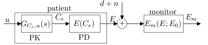
Fig. 2. Combined patient and monitor model with input u , measurement noise n , modeled surgical stimulation d , clinical effect E and measurement E_m .
