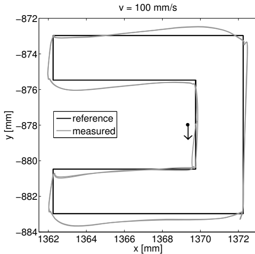
Figure 7.5 Control performance of the robot for low ( v = 10 \text{ mm s}^{-1} , 7.5(a)) and high ( v = 100 \text{ mm s}^{-1} , 7.5(b)) velocity. The motion starts next to the indicated point in negative y -direction. Reference z_r (black) and measured tool position z_m (grey).
