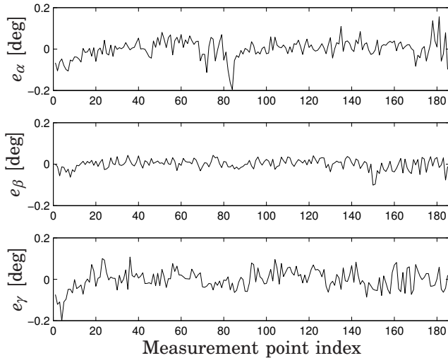
Figure 5.10 Angular errors ( e_\alpha, e_\beta, e_\gamma ) for the identified F1 model, represented in ZYZ Euler angles. The corresponding values for the nominal parameters reached up to 6.7^\circ .
