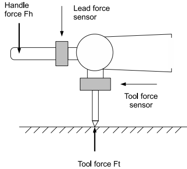
Figure 8.1 Force sensor placement
