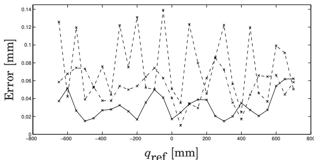
Figure 5.2 Linearity error of the D1 prototype actuators: Absolute value of residuals when fitting a linear function to the movement of cart 1 (solid), cart 2 (dashed) and cart 3 (dashed-dotted). Along the abscissa, the commanded cart position is shown.
