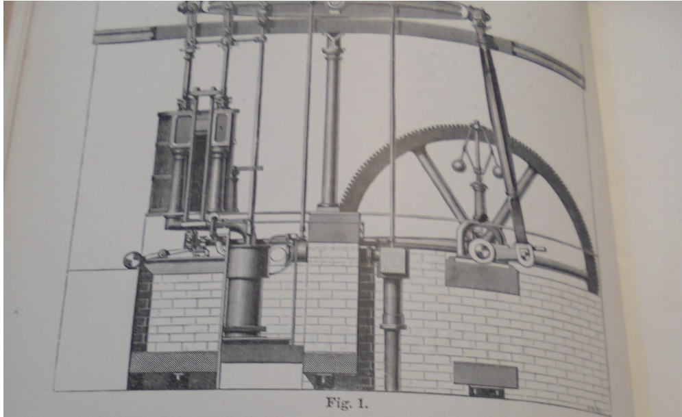
Figure 3: Steam engine offered by Appleby's circa 1878
