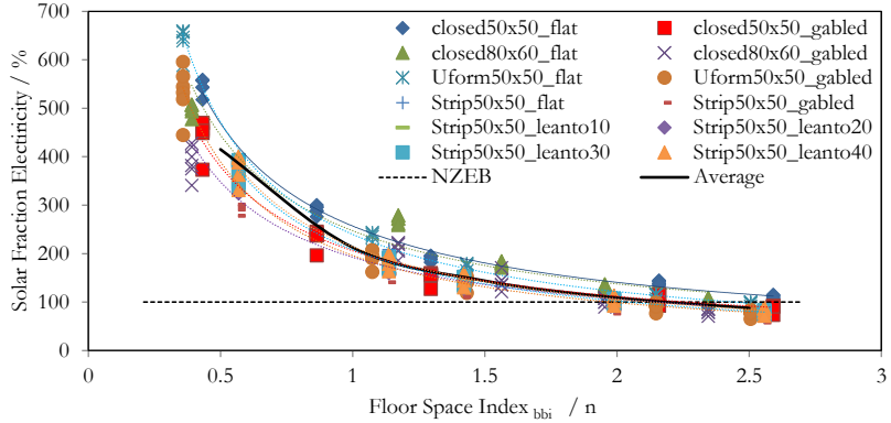
Figure 6.5 FEBY / BBR load matching for electricity demand
