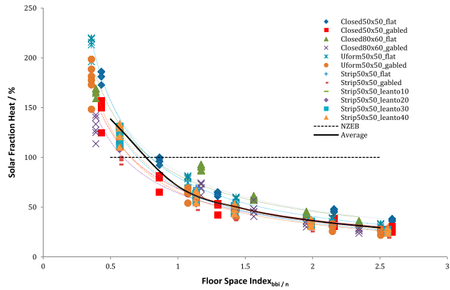
Figure 9. BBR load matching for heating demand.
