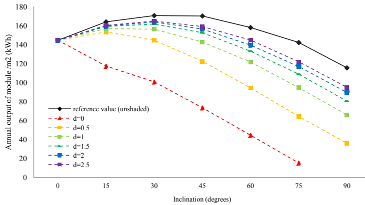
Figure 3. Output of the reference module and the shaded module in Lund.
