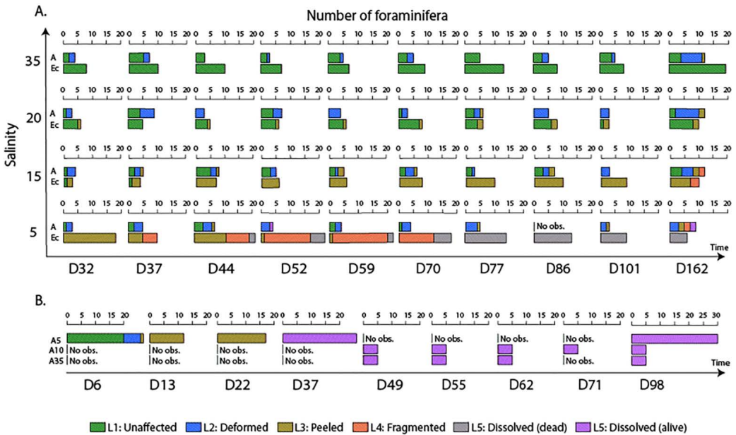
Fig. 4. A. Level of test morphology and dissolution of Ammonia sp. (A) and E. crispum (Ec) at different salinities and times. Note that, except at day 162, the number of foraminifera does not refer to the total amount of foraminifera present but to the number of observed specimens at a given time. B. Level of test morphology and dissolution of juveniles Ammonia sp. at salinity 5 (A5), 10 (A10) and 35 (A35).
