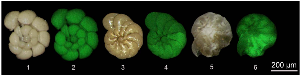
Plate 3. Living decalcified foraminifera in DCHa-2, the same specimens are shown under normal light and epifluorescent light. 1-2: Ammonia sp. 3-4: Elphidium sp. 5-6: half decalcified Elphidium sp.
